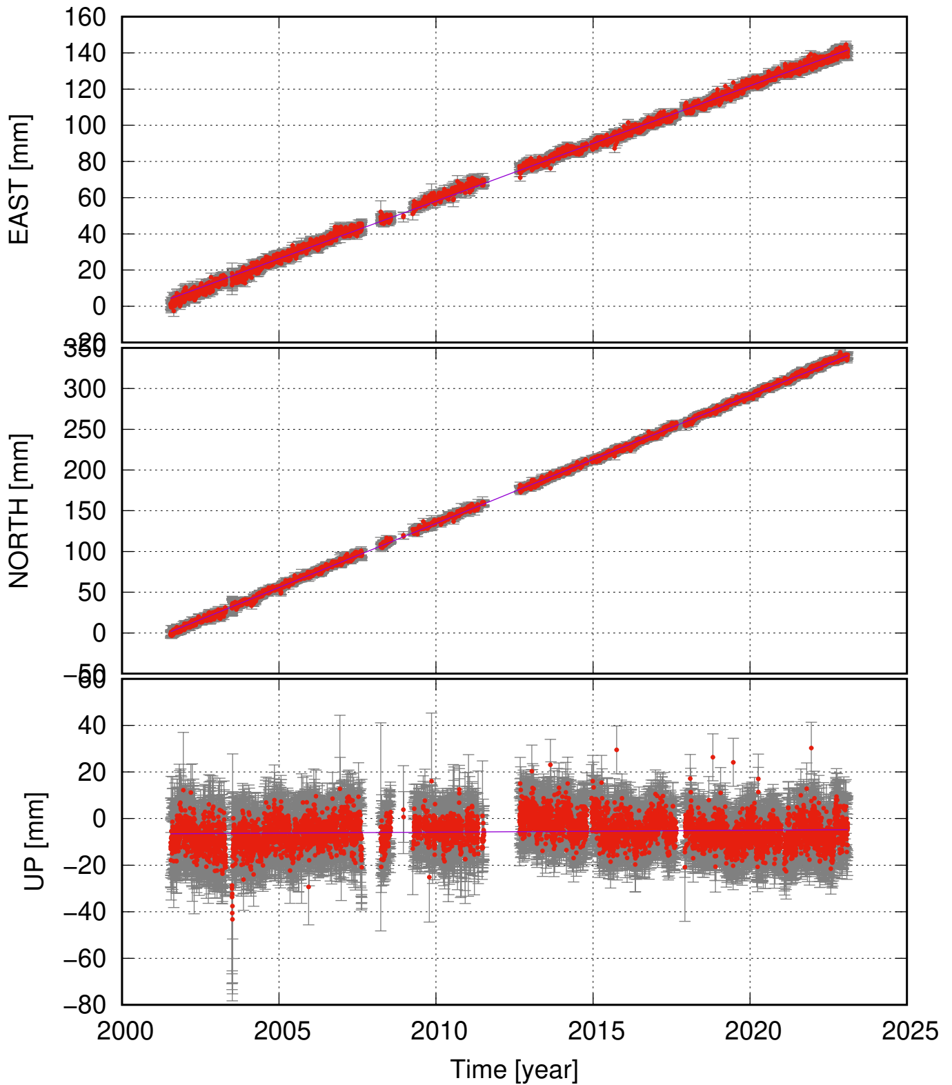
RHOF (66.46, -15.95) time series (ITRF 2014) v_e = 6.37 \pm 0.08 ; v_n = 15.72 \pm 0.09 ; v_u = 0.08 \pm 0.27 mm/yr
