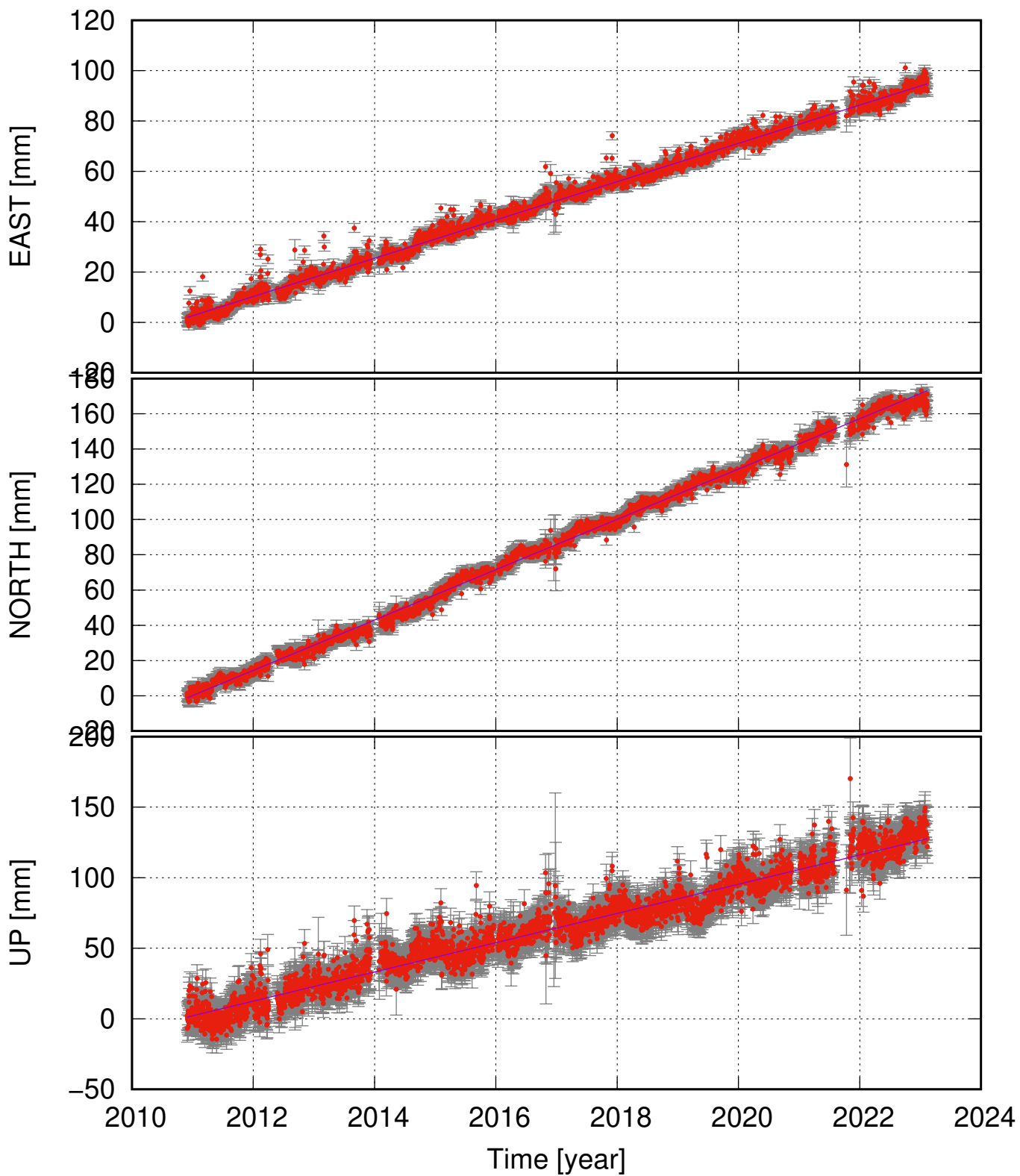
RFEL (63.62, -18.67) time series (ITRF 2014) v_e = 7.61 \pm 0.17 ; v_n = 14.28 \pm 0.23 ; v_u = 10.36 \pm 0.65 mm/yr
