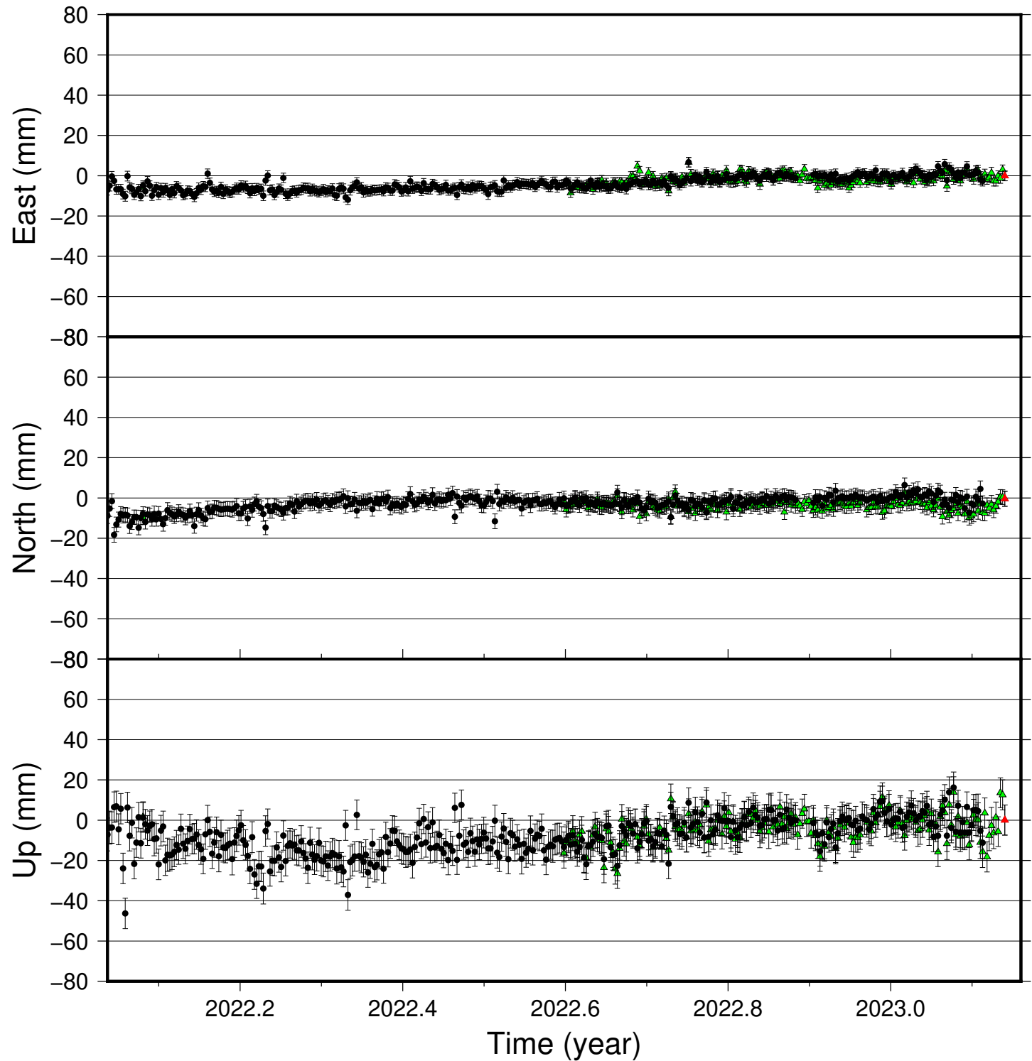
RFEL time series (IGS 2014), last 400 days
