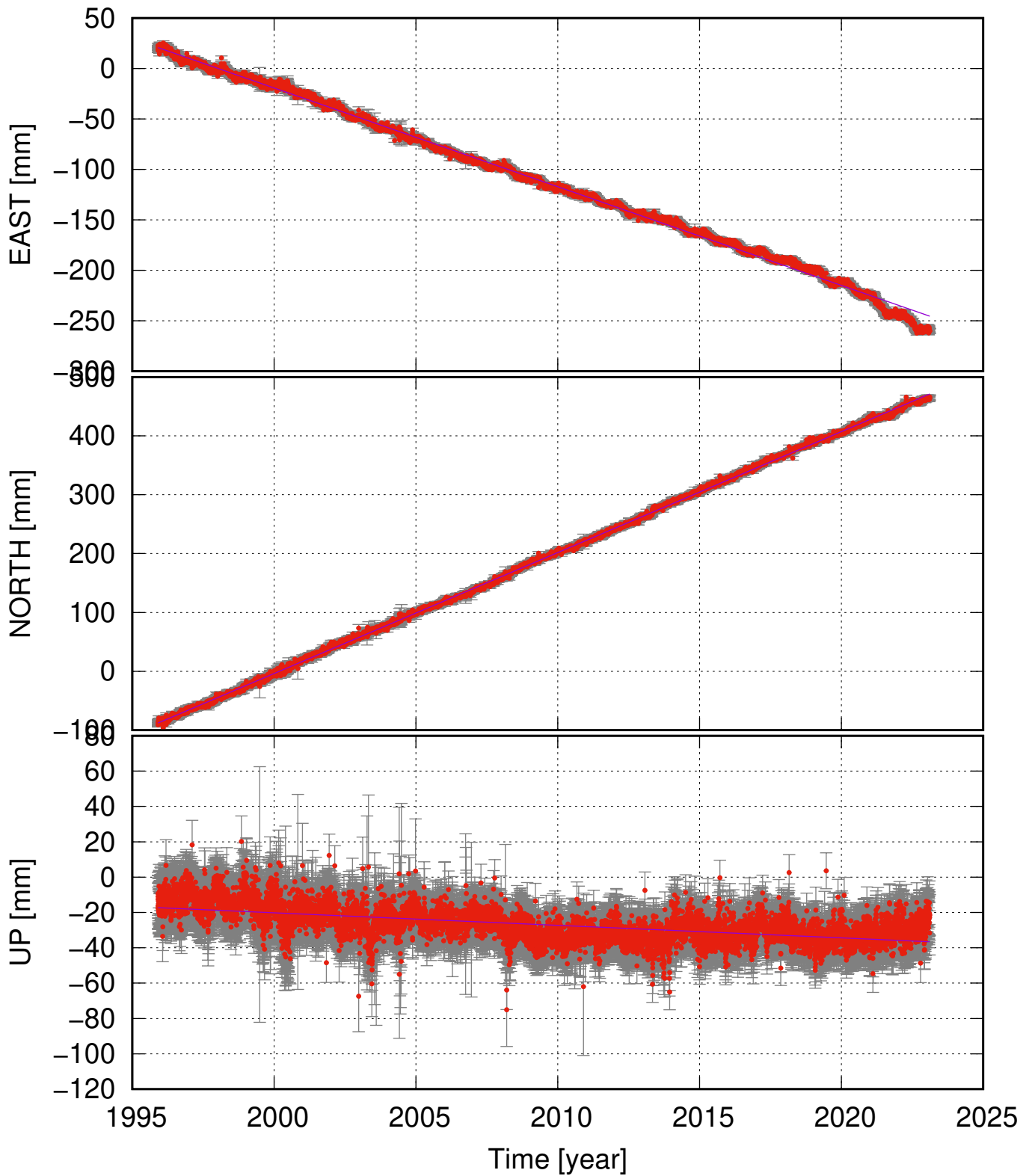
REYK (64.14, -21.96) time series (ITRF 2014) v_e = -9.79 \pm 0.16 ; v_n = 20.55 \pm 0.11 ; v_u = -0.71 \pm 0.26 mm/yr
