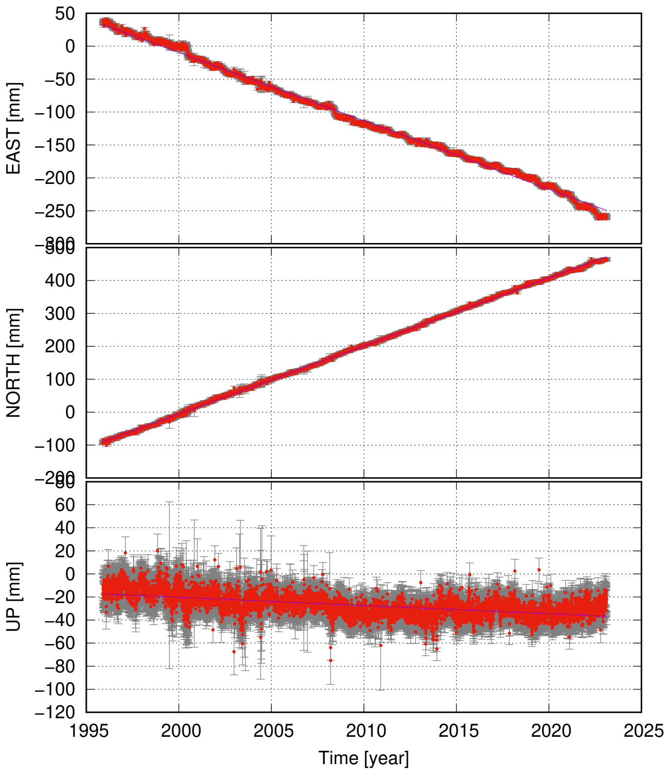
REYK (64.14, -21.96) time series (ITRF 2014) ve = -10.38 \pm 0.18 ; vn = 20.65 \pm 0.13 ; vu = -0.71 \pm 0.26 mm/yr
