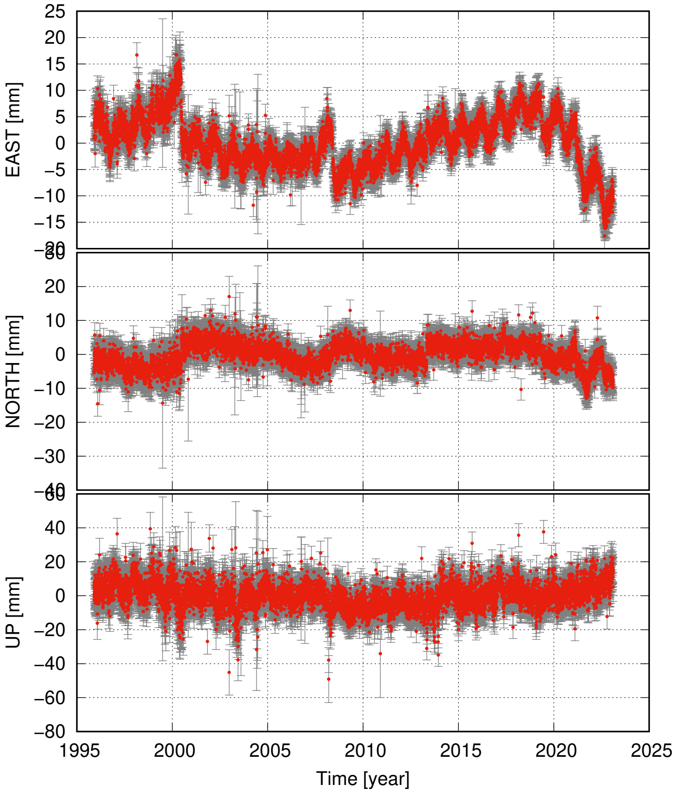
REYK residual time series
