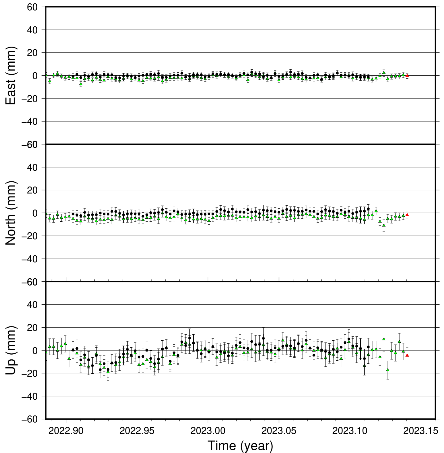
REYK time series (IGS 2014), last 100 days
