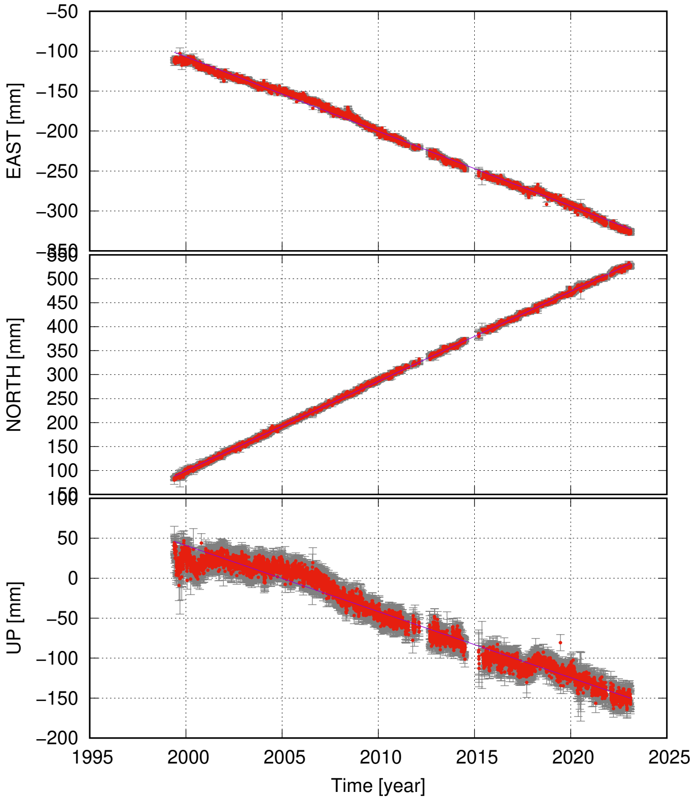
OLKE (64.06, -21.22) time series (ITRF 2014) v_e = -9.34 \pm 0.15 ; v_n = 18.71 \pm 0.10 ; v_u = -8.27 \pm 0.42 mm/yr
