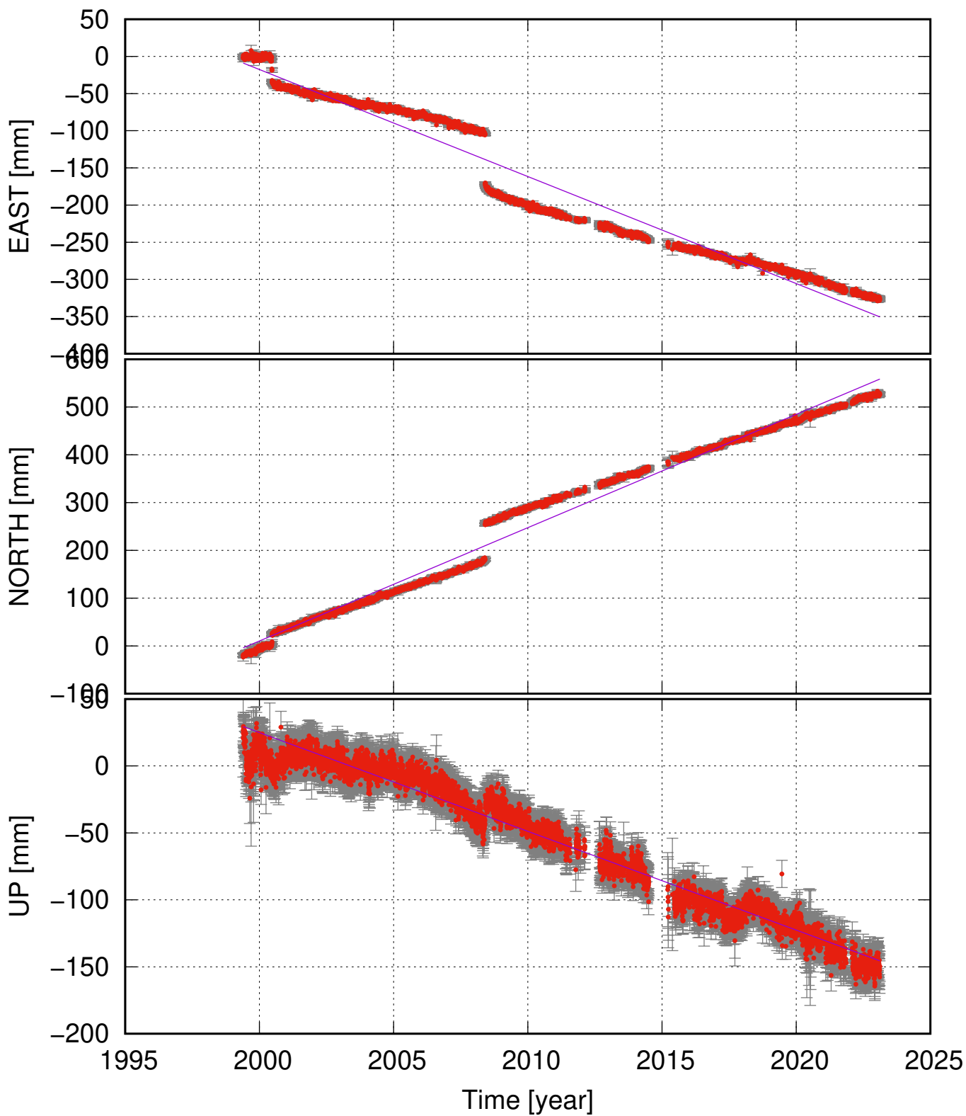
OLKE (64.06, -21.22) time series (ITRF 2014) v_e = -14.40 \pm 0.92 ; v_n = 23.72 \pm 0.93 ; v_u = -7.38 \pm 0.39 mm/yr
