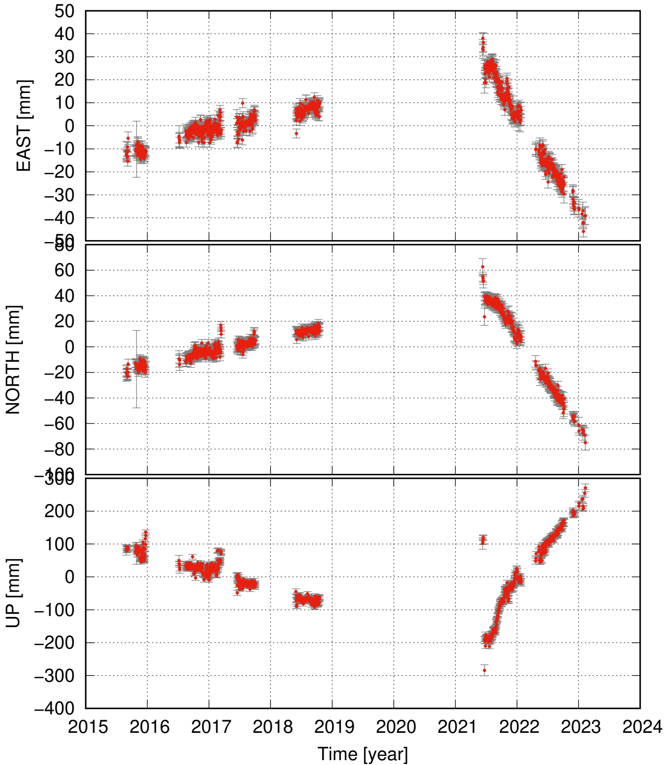
OLAC residual time series (some major events removed as well)
