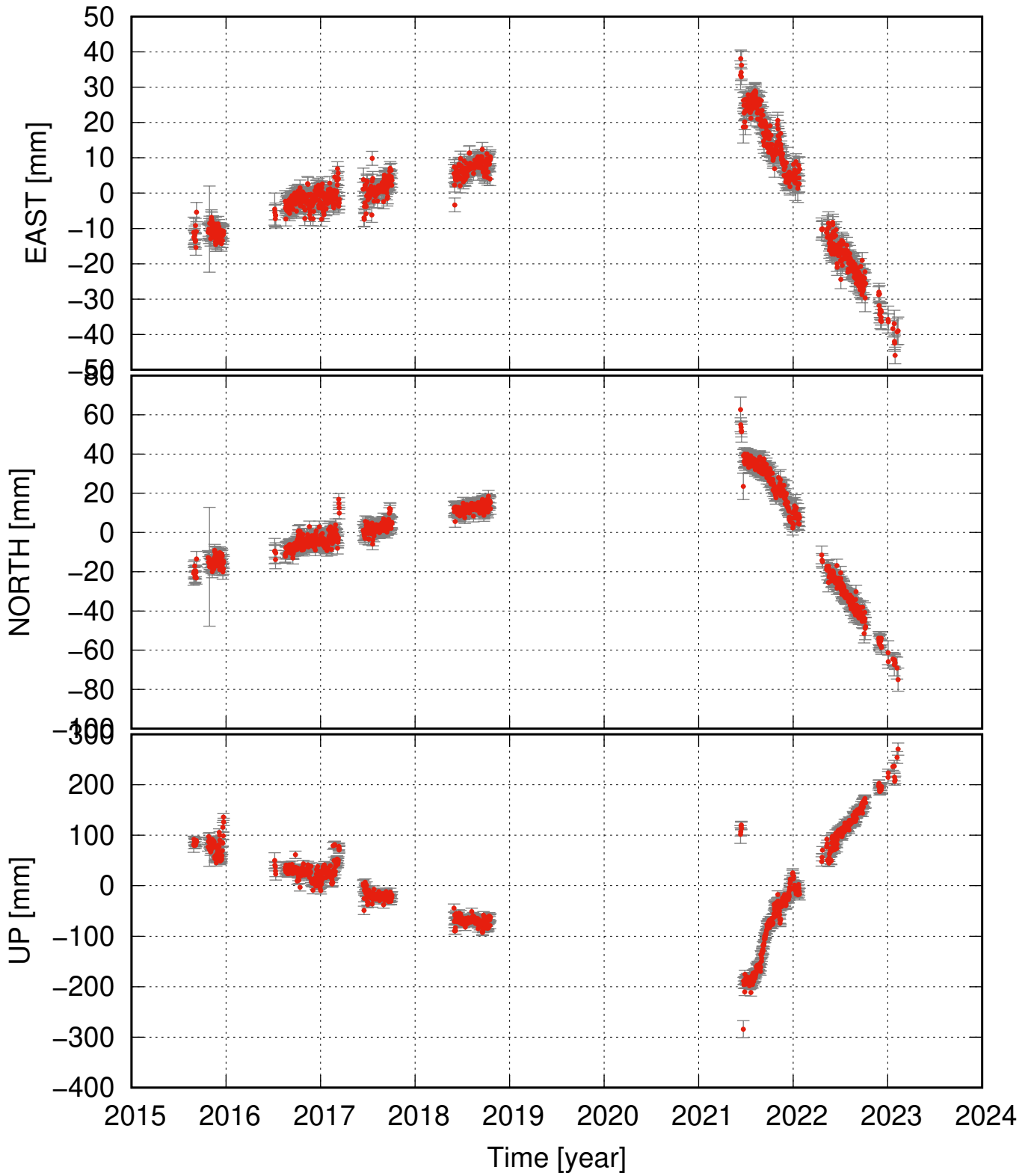
OLAC residual time series
