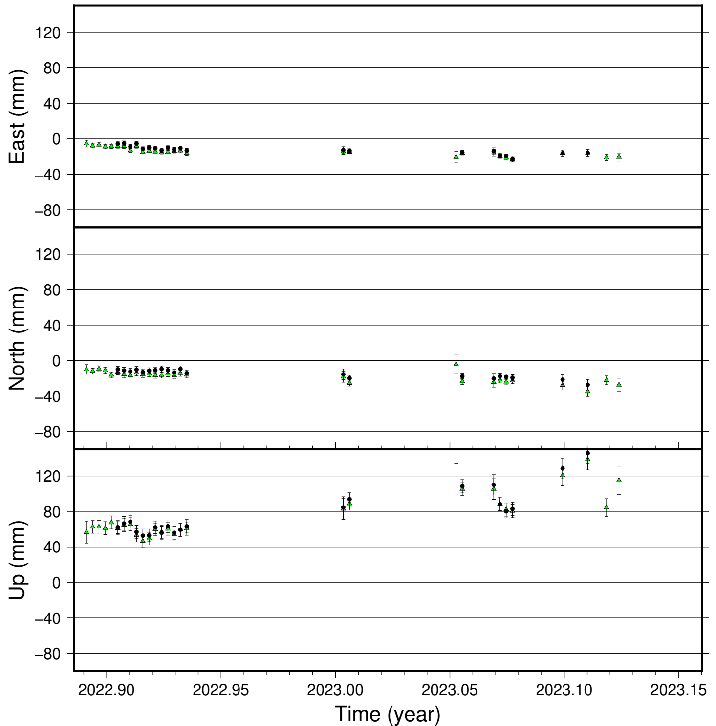
OLAC time series (IGS 2014), last 100 days
