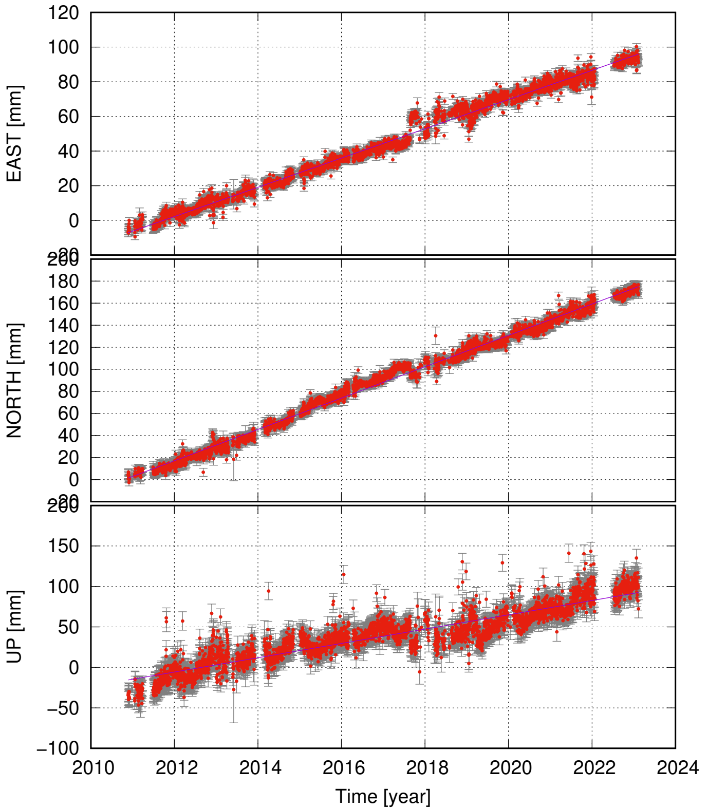
OFEL (63.75, -18.84) time series (ITRF 2014) v_e = 8.43 \pm 0.25 ; v_n = 14.21 \pm 0.36 ; v_u = 8.83 \pm 1.06 mm/yr
