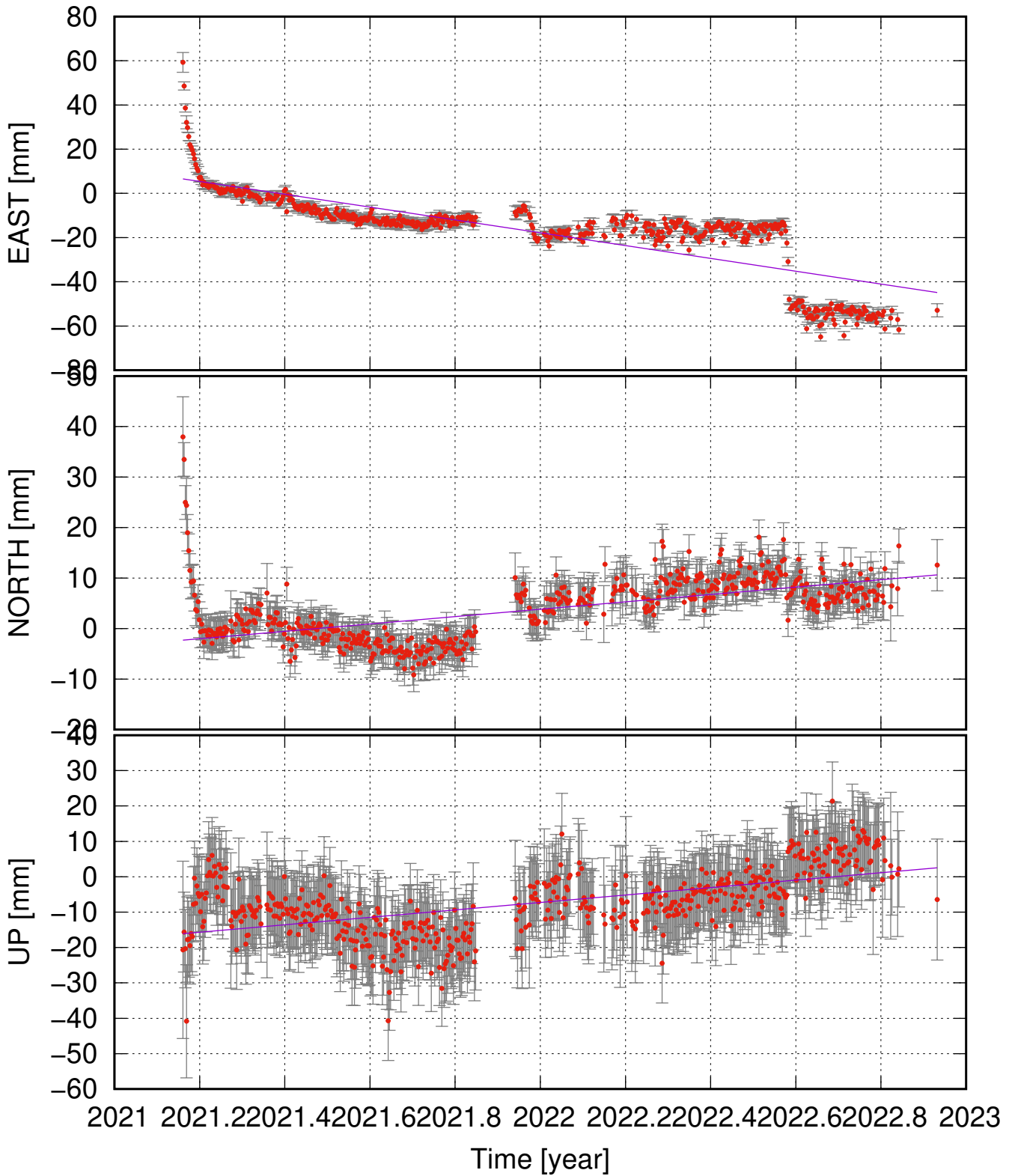
ODDF (63.95, -22.12) time series (ITRF 2014) ve = -29.02 ± 6.11; vn = 7.28 ± 2.83; vu = 10.50 ± 4.20 mm/yr
