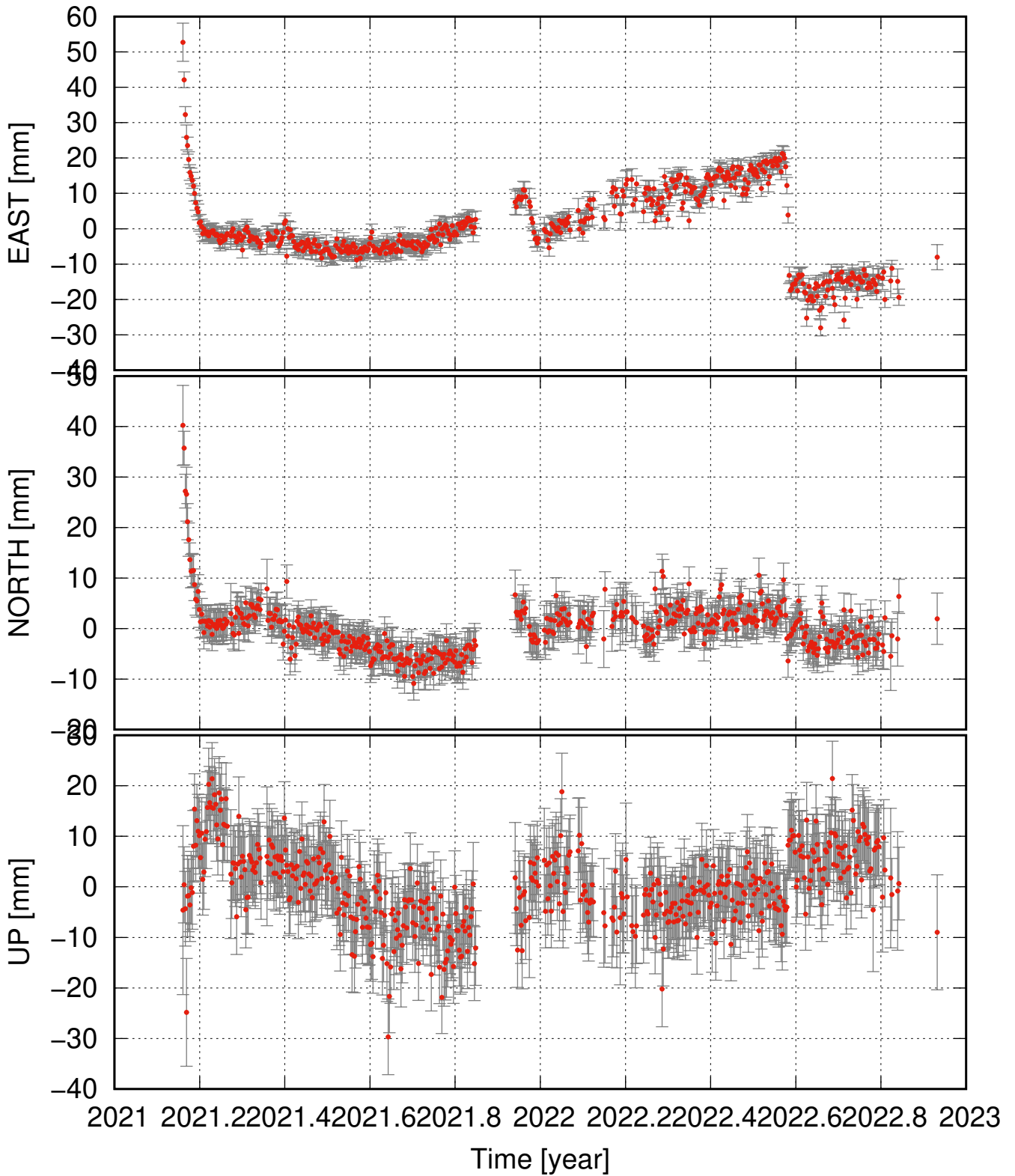
ODDF residual time series (some major events removed as well)
