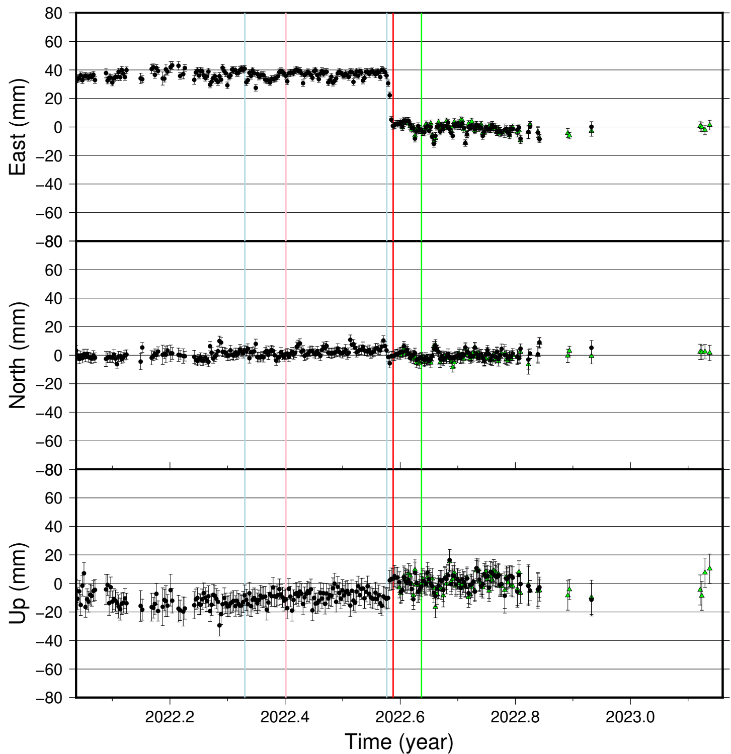
ODDF time series (IGS 2014), last 400 days
