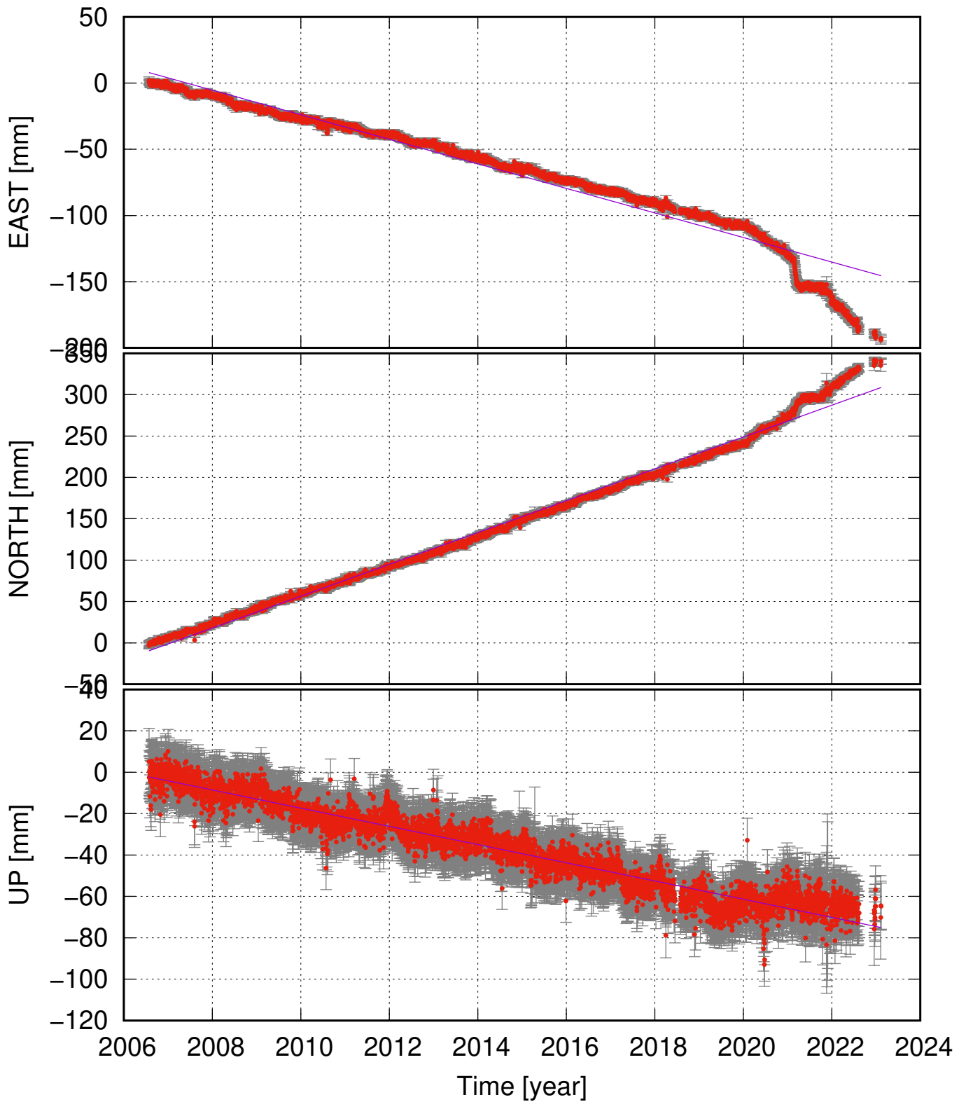
NYLA (63.97, -22.74) time series (ITRF 2014) ve = -9.27 \pm 0.63 ; vn = 19.24 \pm 0.51 ; vu = -4.40 \pm 0.33 mm/yr
