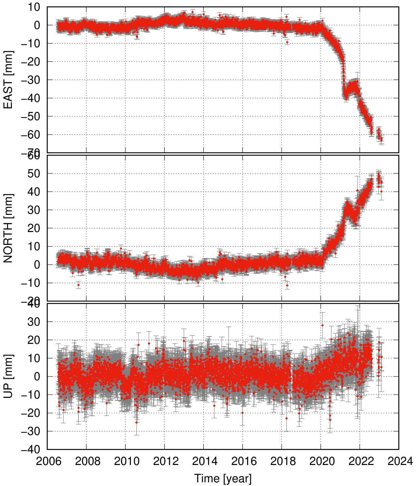
NYLA detrended and seasonal signal removed
