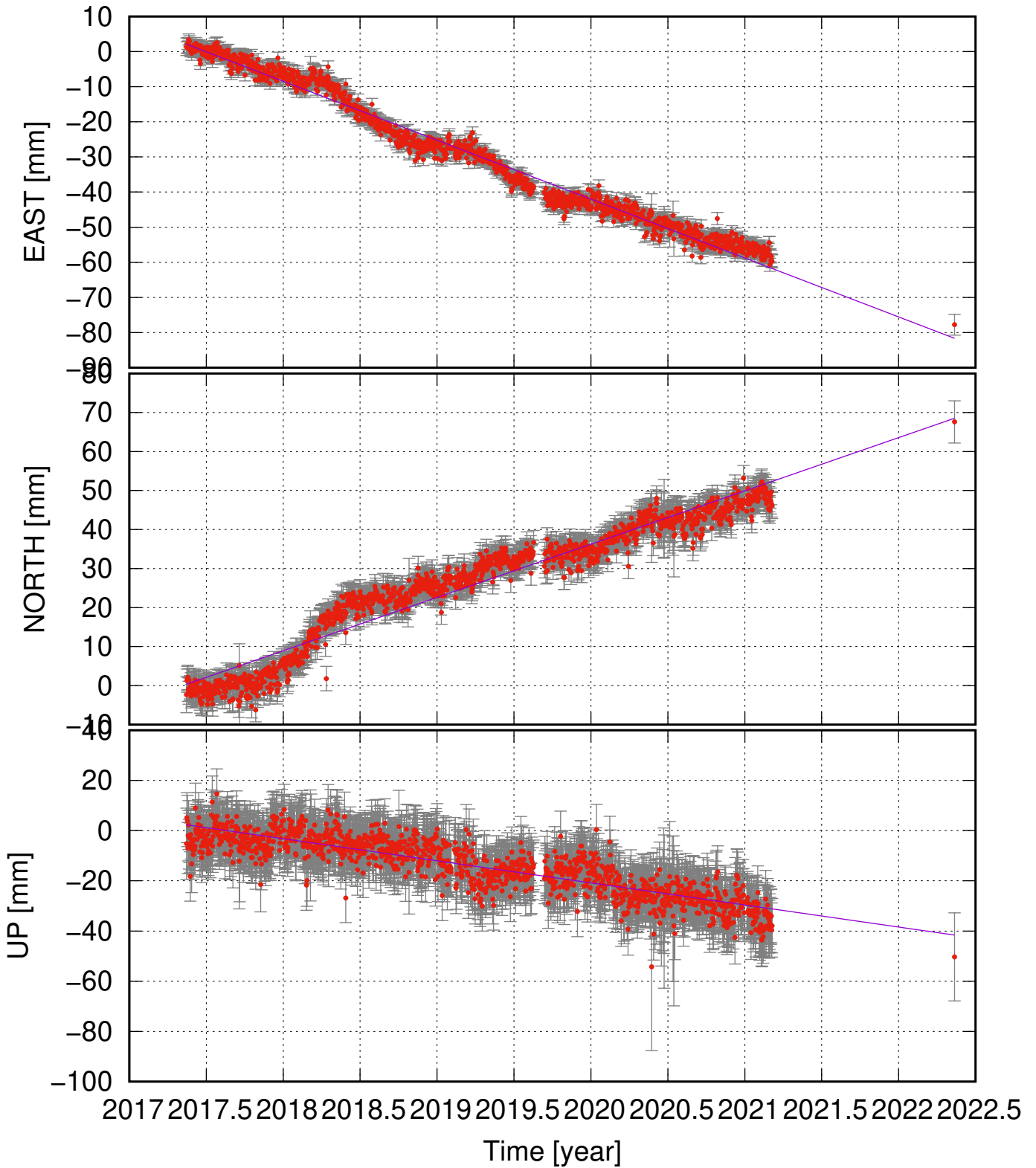
NVEL (64.11, -21.25) time series (ITRF 2014) v_e = -16.79 \pm 0.52 ; v_n = 13.65 \pm 0.78 ; v_u = -8.80 \pm 1.10 mm/yr
