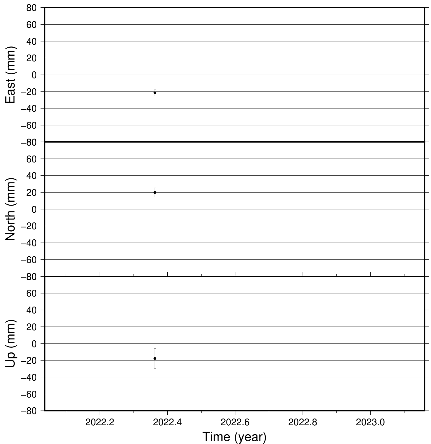
NVEL time series (IGS 2014), last 400 days
