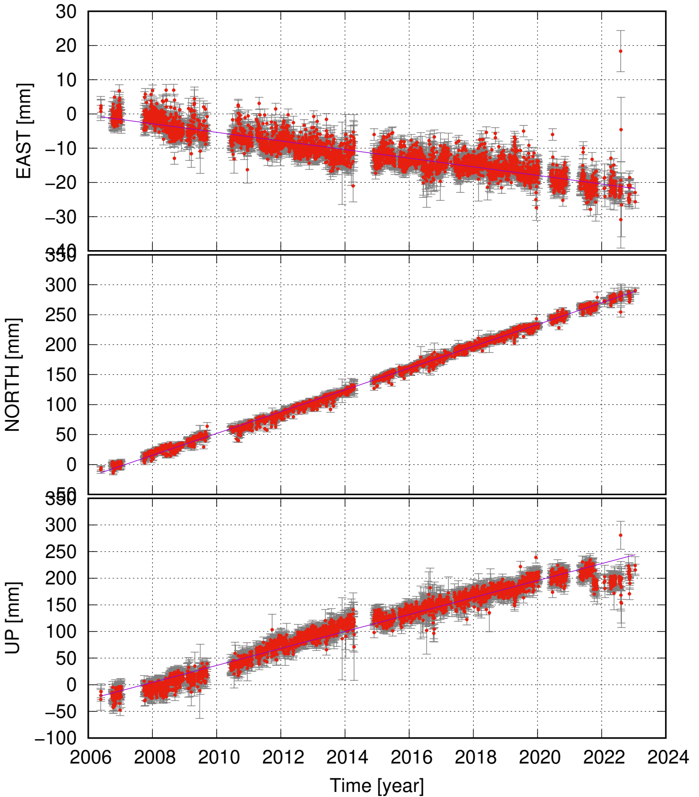
NORS (64.03, -19.72) time series (ITRF 2014) v_e = -1.26 \pm 0.15 ; v_n = 18.19 \pm 0.25 ; v_u = 15.94 \pm 0.76 mm/yr
