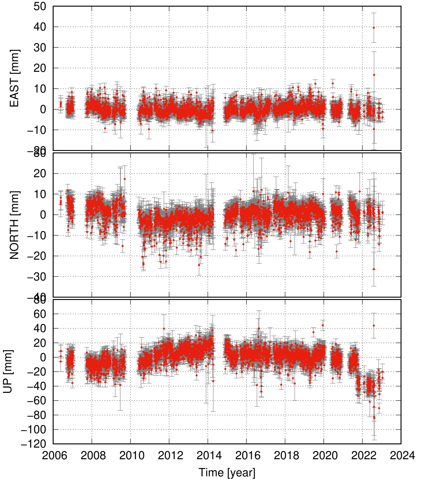
NORS residual time series
