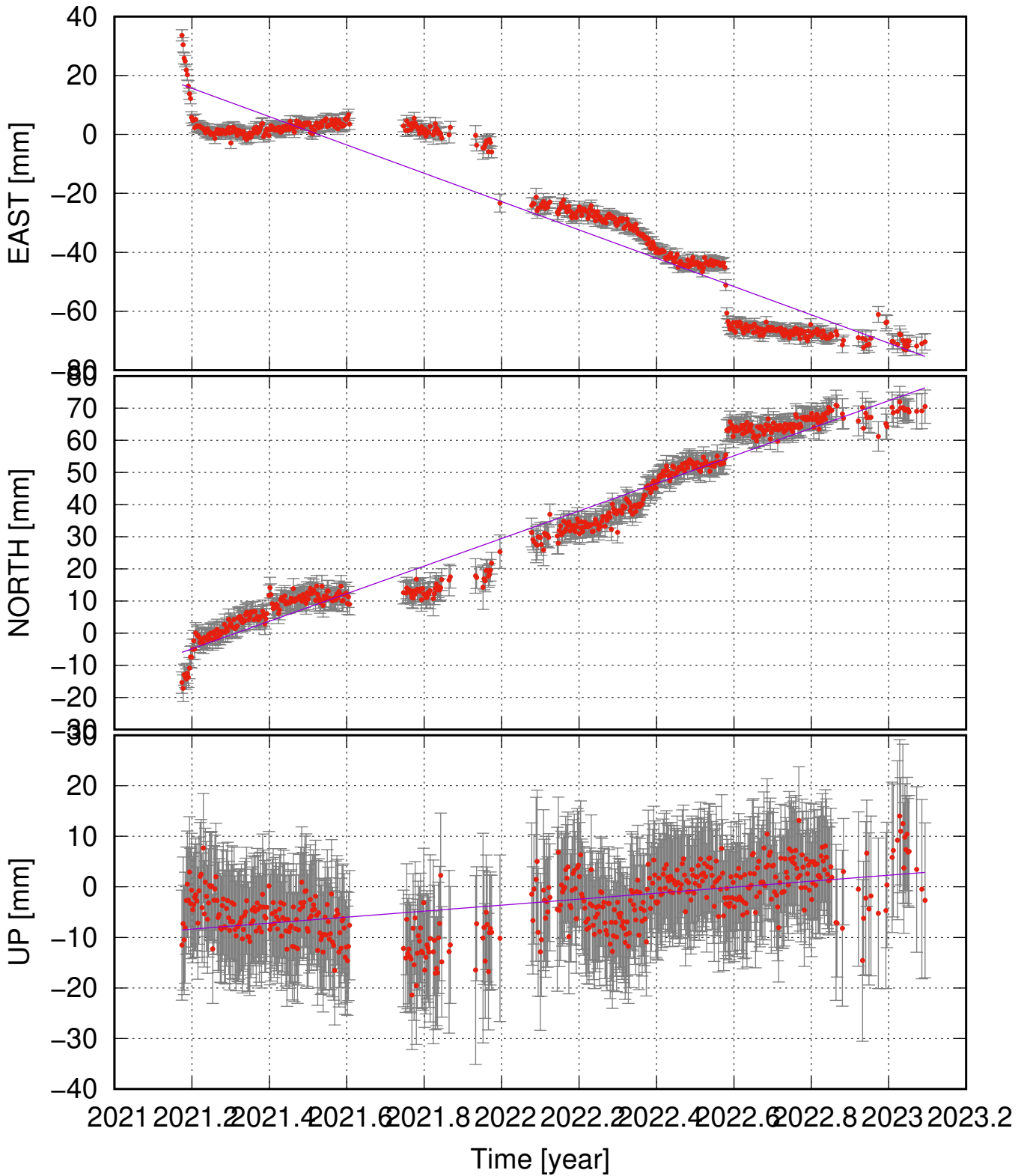
NAMC (63.92, -22.54) time series (ITRF 2014) v_e = -48.04 \pm 4.42 ; v_n = 42.87 \pm 2.48 ; v_u = 5.91 \pm 2.59 mm/yr
