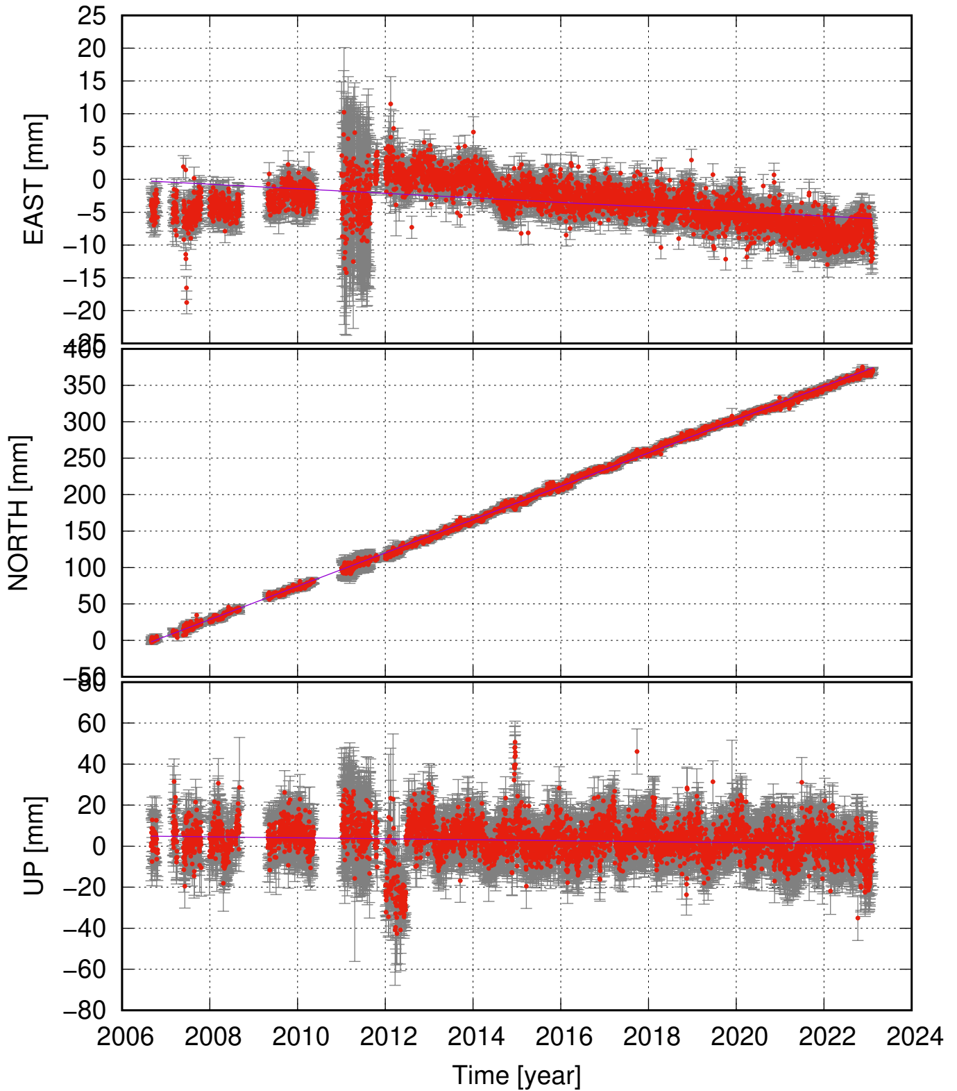
MYVA (65.64, -16.89) time series (ITRF 2014) v_e = -0.35 \pm 0.16 ; v_n = 22.86 \pm 0.17 ; v_u = -0.24 \pm 0.51 mm/yr
