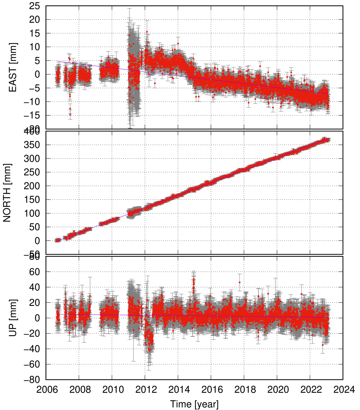
MYVA (65.64, -16.89) time series (ITRF 2014) v_e = -0.72 \pm 0.18 ; v_n = 22.86 \pm 0.17 ; v_u = -0.24 \pm 0.51 mm/yr
