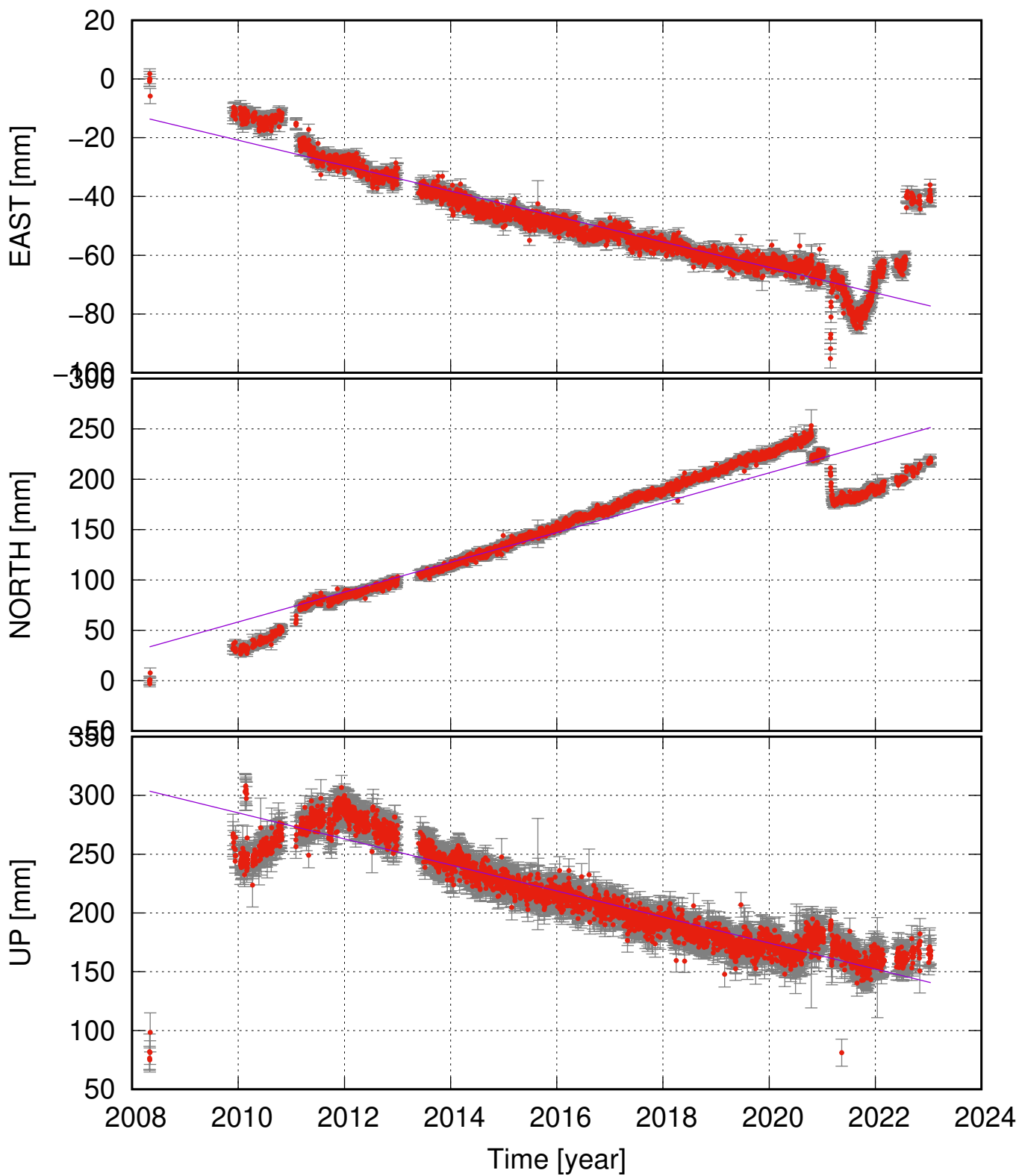
MOHA (63.92, -22.06) time series (ITRF 2014) v_e = -4.33 \pm 0.38 ; v_n = 14.81 \pm 1.33 ; v_u = -11.06 \pm 1.01 mm/yr
