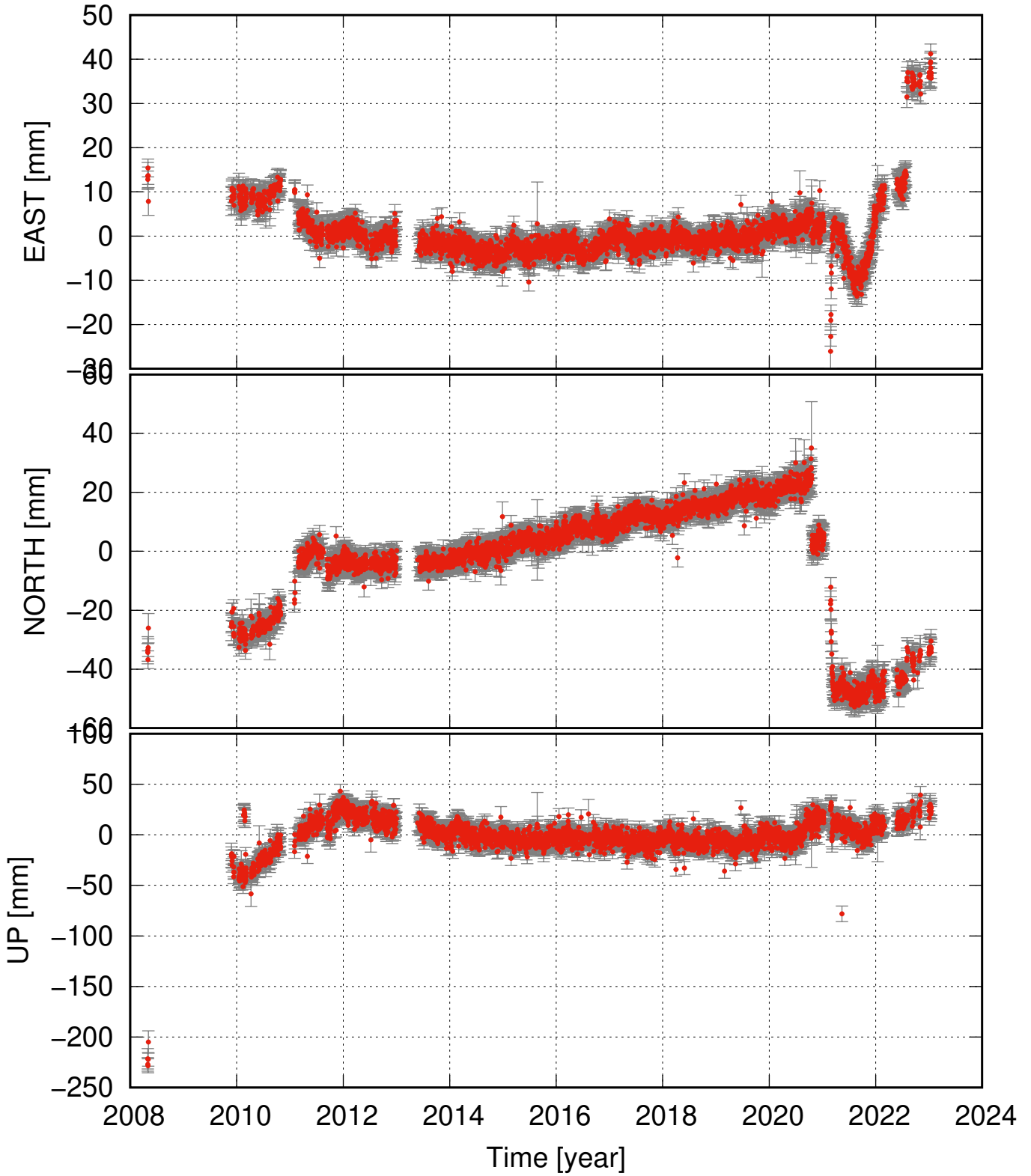
MOHA residual time series (some major events removed as well)
