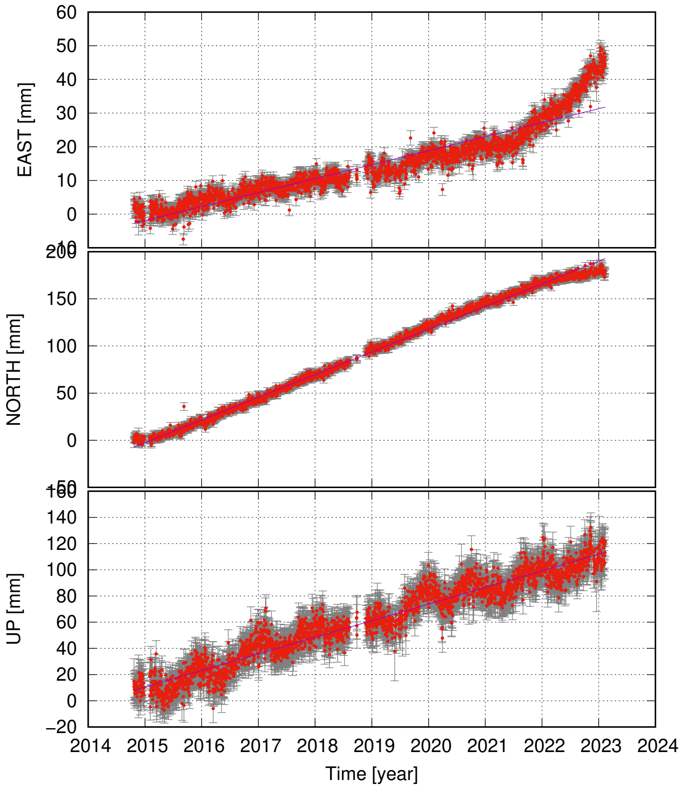
MOFC (64.98, -16.67) time series (ITRF 2014) v_e = 4.15 \pm 0.46 ; v_n = 24.07 \pm 0.48 ; v_u = 12.67 \pm 0.99 mm/yr
