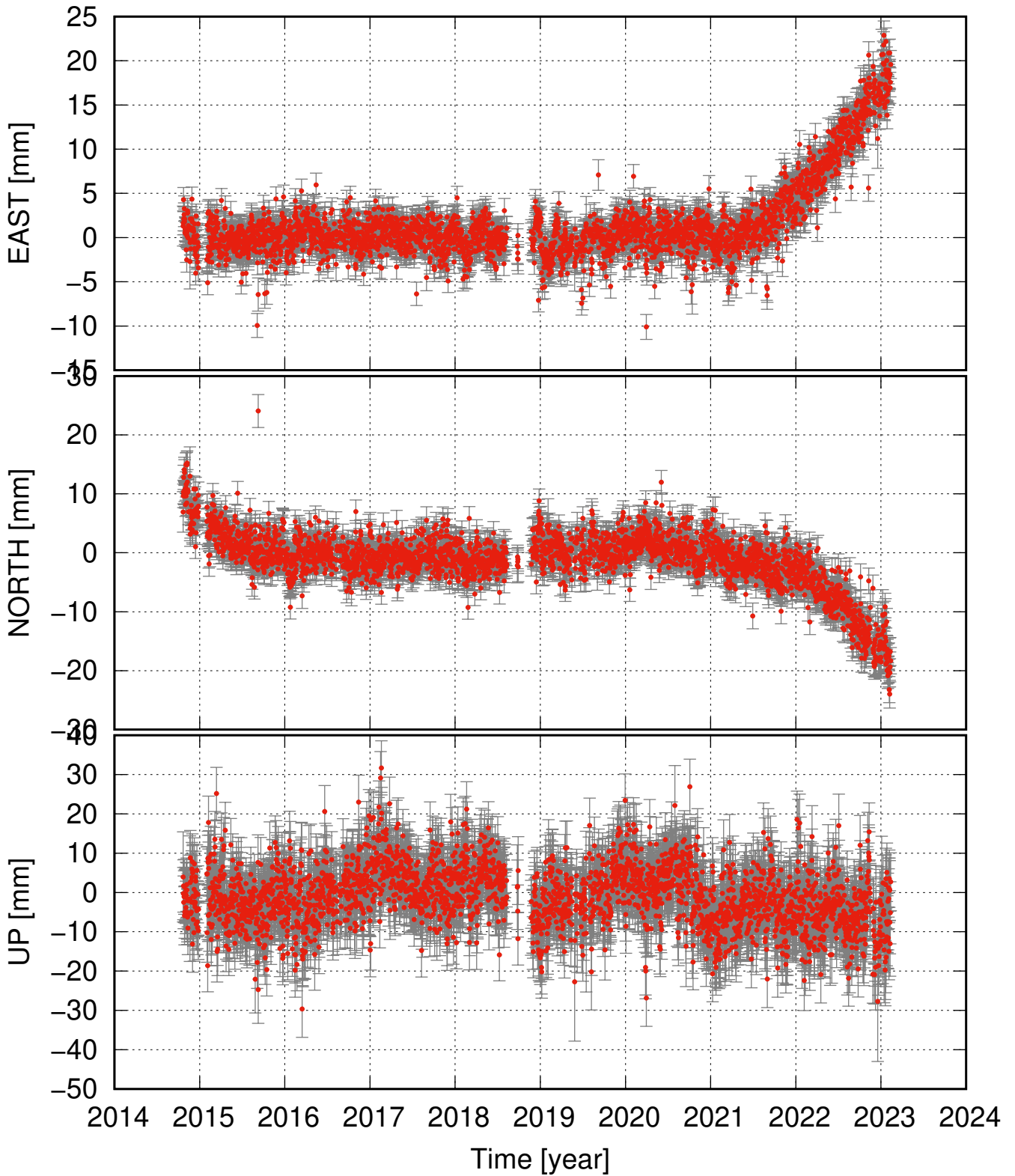
MOFC detrended and seasonal signal removed
