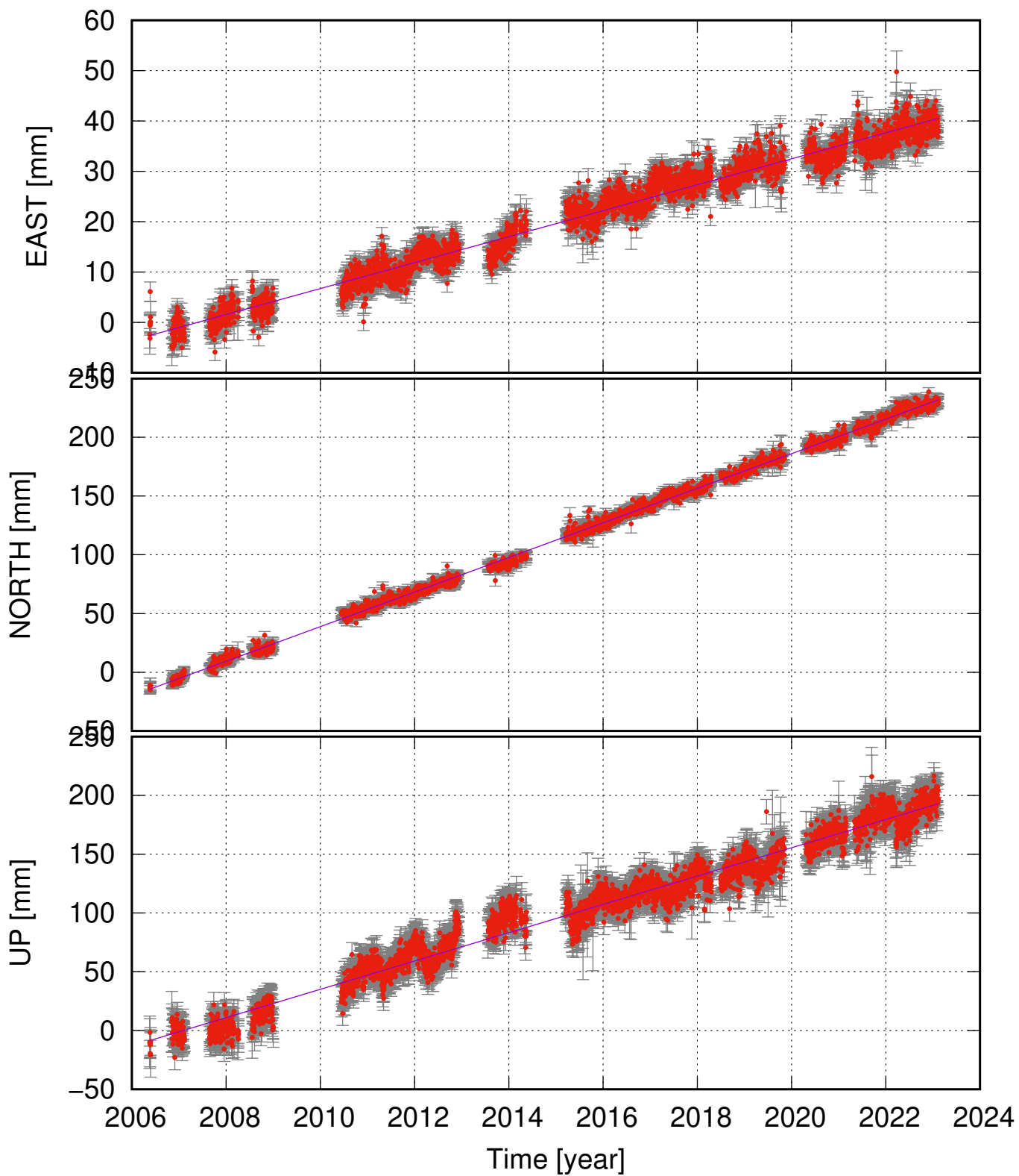
MJSK (63.93, -19.67) time series (ITRF 2014) v_e = 2.58 \pm 0.12 ; v_n = 14.72 \pm 0.18 ; v_u = 12.04 \pm 0.57 mm/yr
