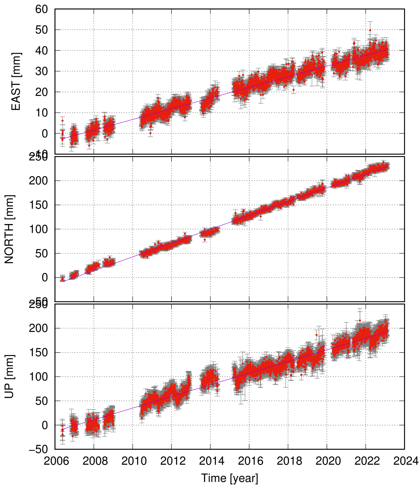
MJSK (63.93, -19.67) time series (ITRF 2014) v_e = 2.58 \pm 0.12 ; v_n = 14.25 \pm 0.24 ; v_u = 12.04 \pm 0.57 mm/yr
