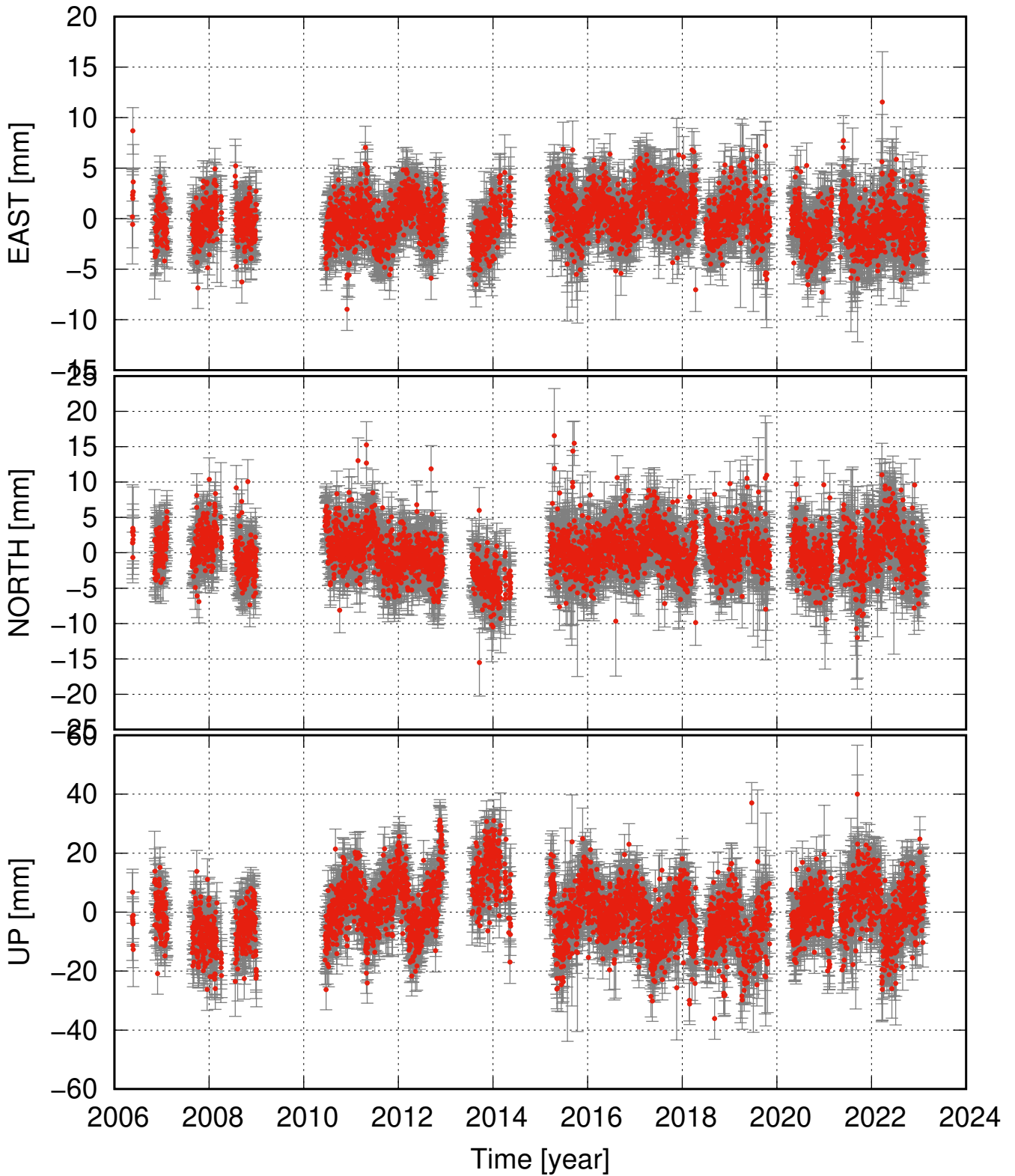
MJSK residual time series (some major events removed as well)
