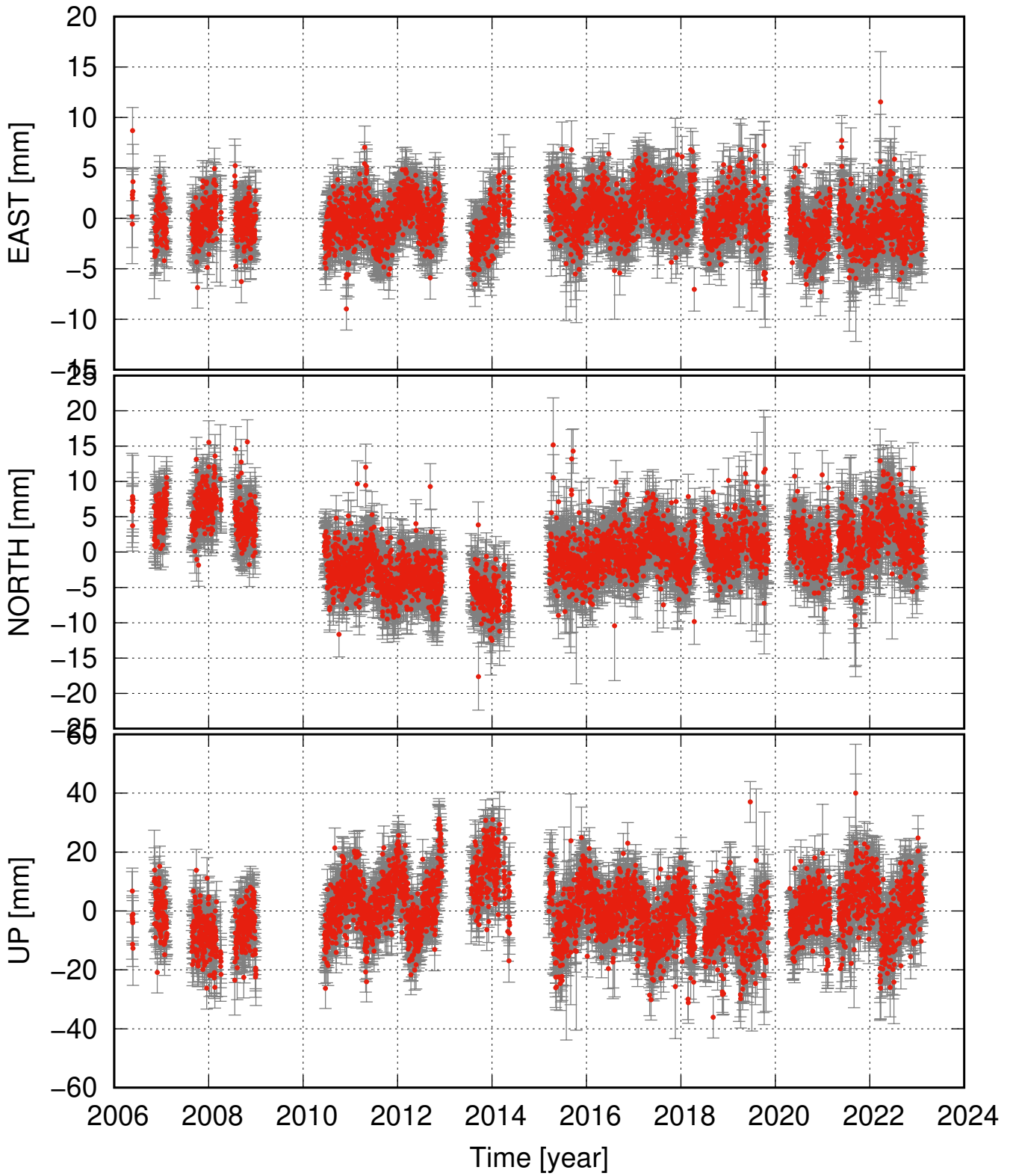
MJSK residual time series
