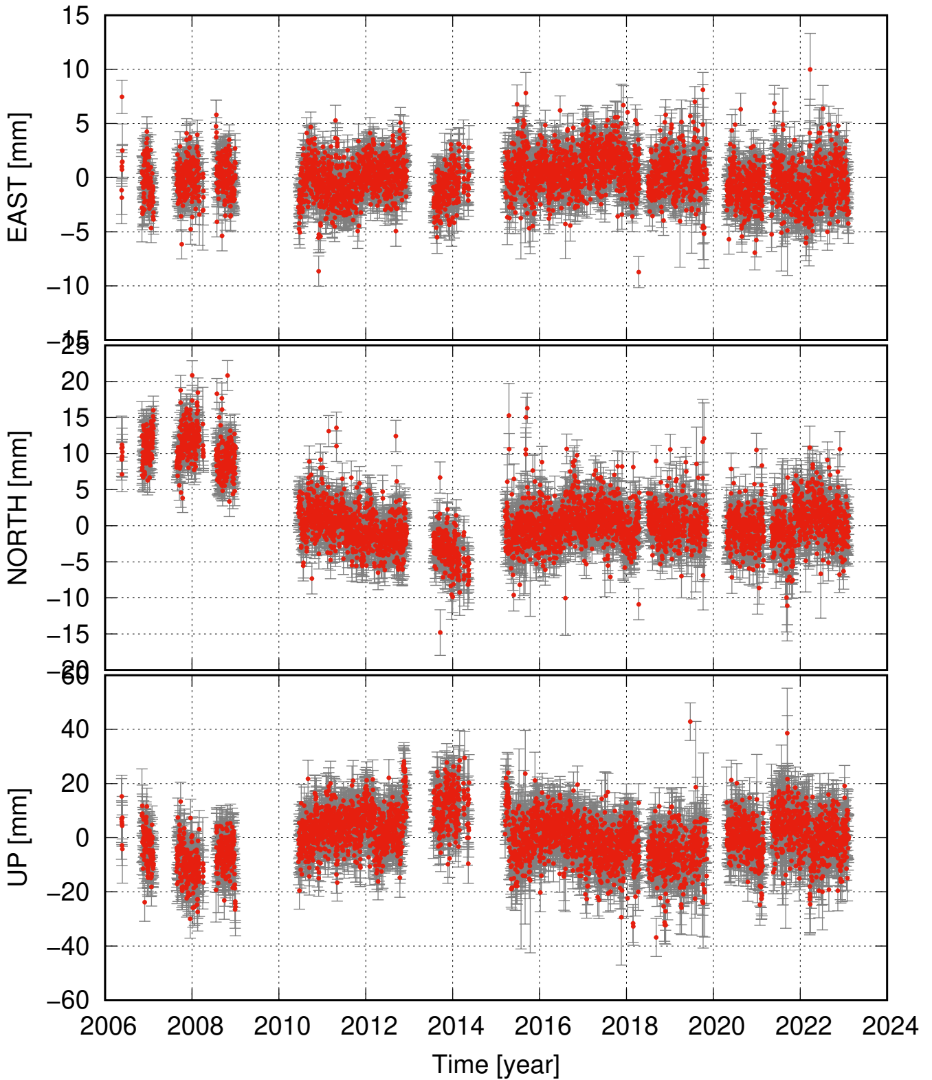
MJSK detrended and seasonal signal removed
