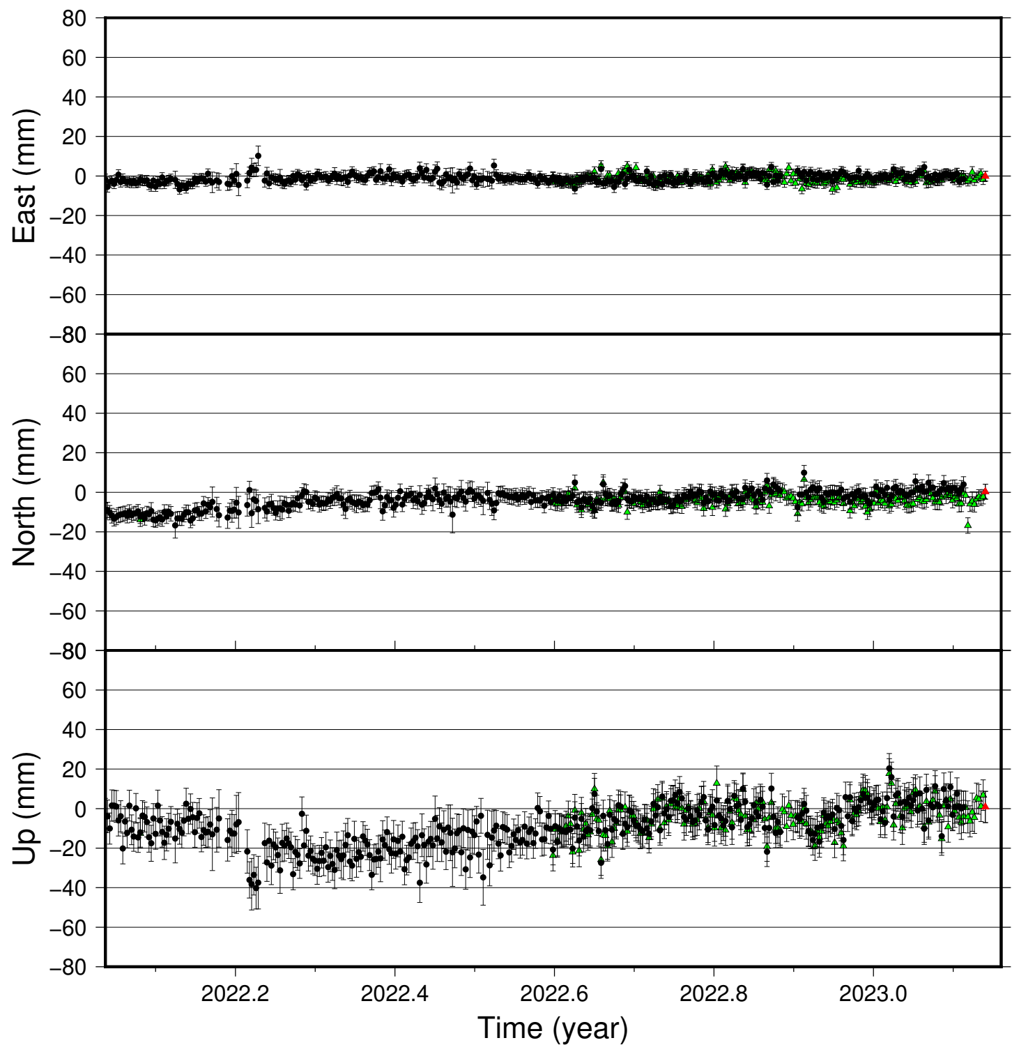
MJSK time series (IGS 2014), last 400 days
