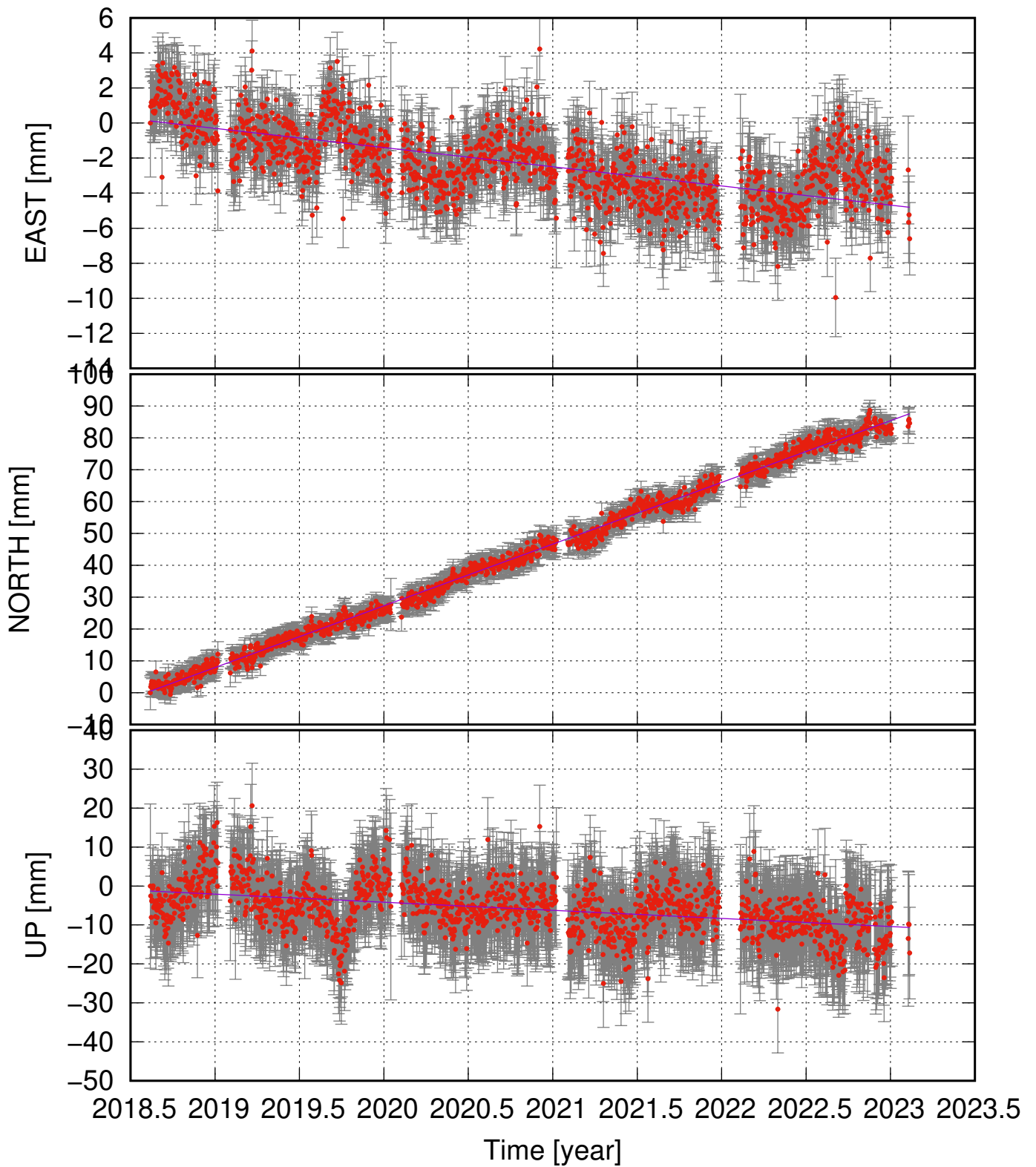
MANA (66.30, -17.12) time series (ITRF 2014) v_e = -1.10 \pm 0.35 ; v_n = 19.37 \pm 0.40 ; v_u = -2.09 \pm 1.24 mm/yr
