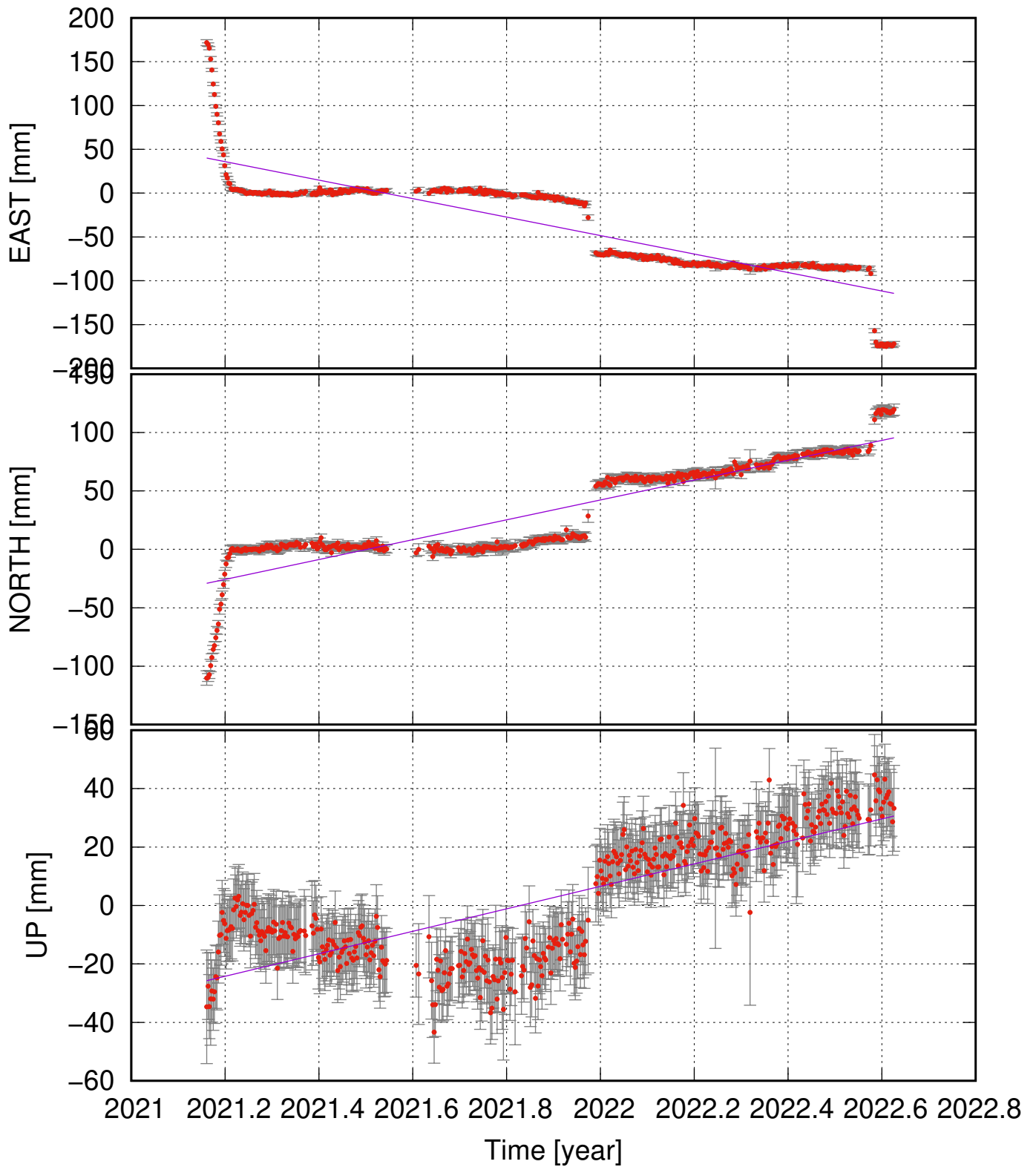
LSK (63.92, -22.37) time series (ITRF 2014) v_e = -105.53 \pm 17.76 ; v_n = 84.97 \pm 11.92 ; v_u = 38.47 \pm 8.60 mm/yr
