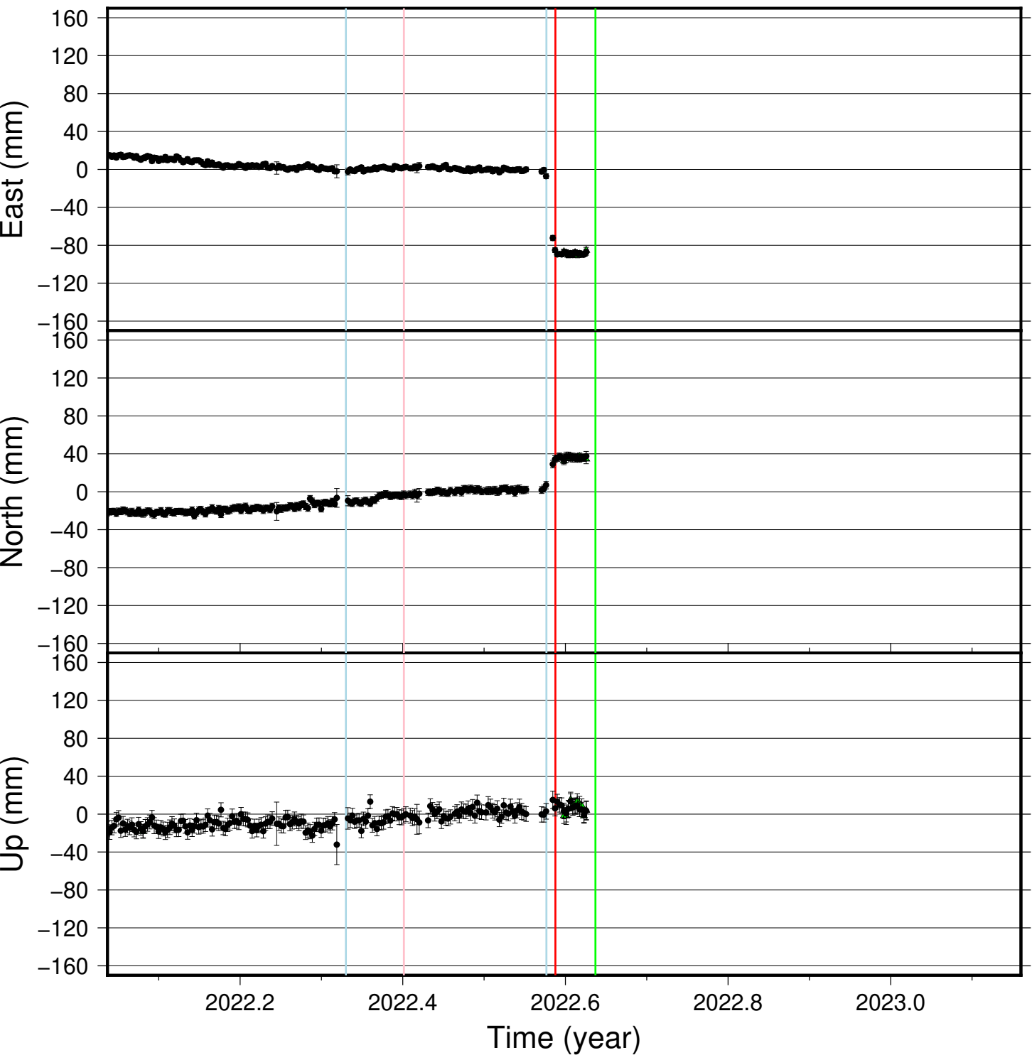
LISK time series (IGS 2014), last 400 days
