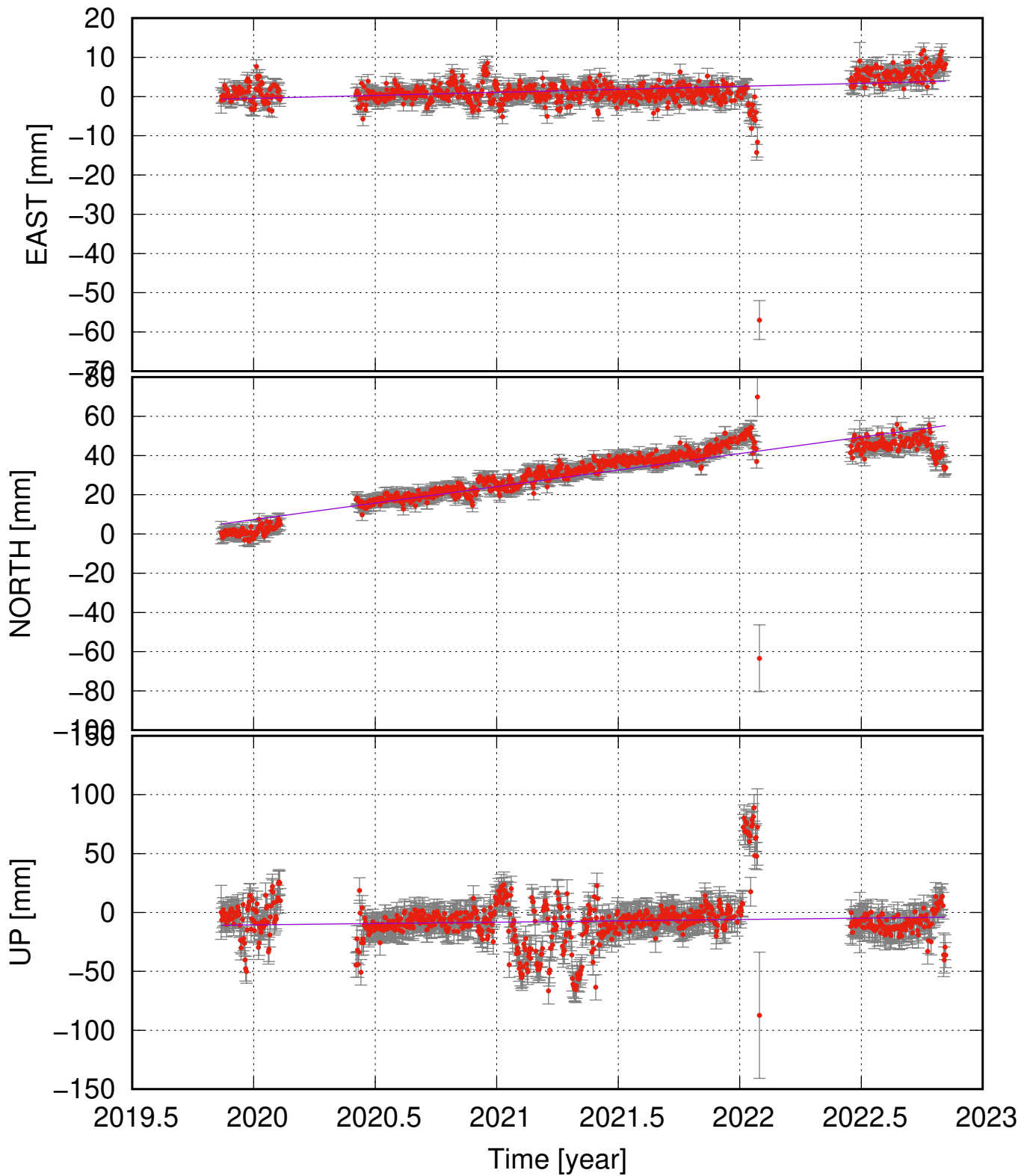
LHNC (65.72, -16.78) time series (ITRF 2014) v_e = 1.55 \pm 1.10 ; v_n = 16.82 \pm 2.14 ; v_u = 2.23 \pm 6.46 mm/yr
