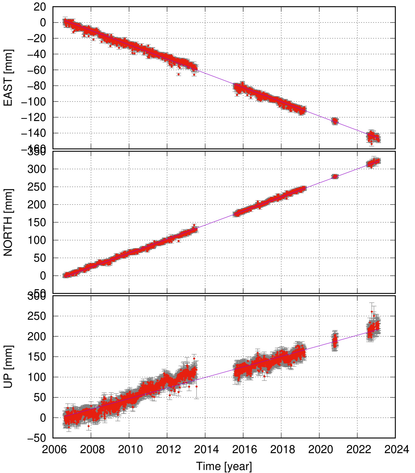
LFEL (64.53, -19.76) time series (ITRF 2014) v_e = -9.03 \pm 0.14 ; v_n = 19.74 \pm 0.18 ; v_u = 12.98 \pm 0.72 mm/yr
