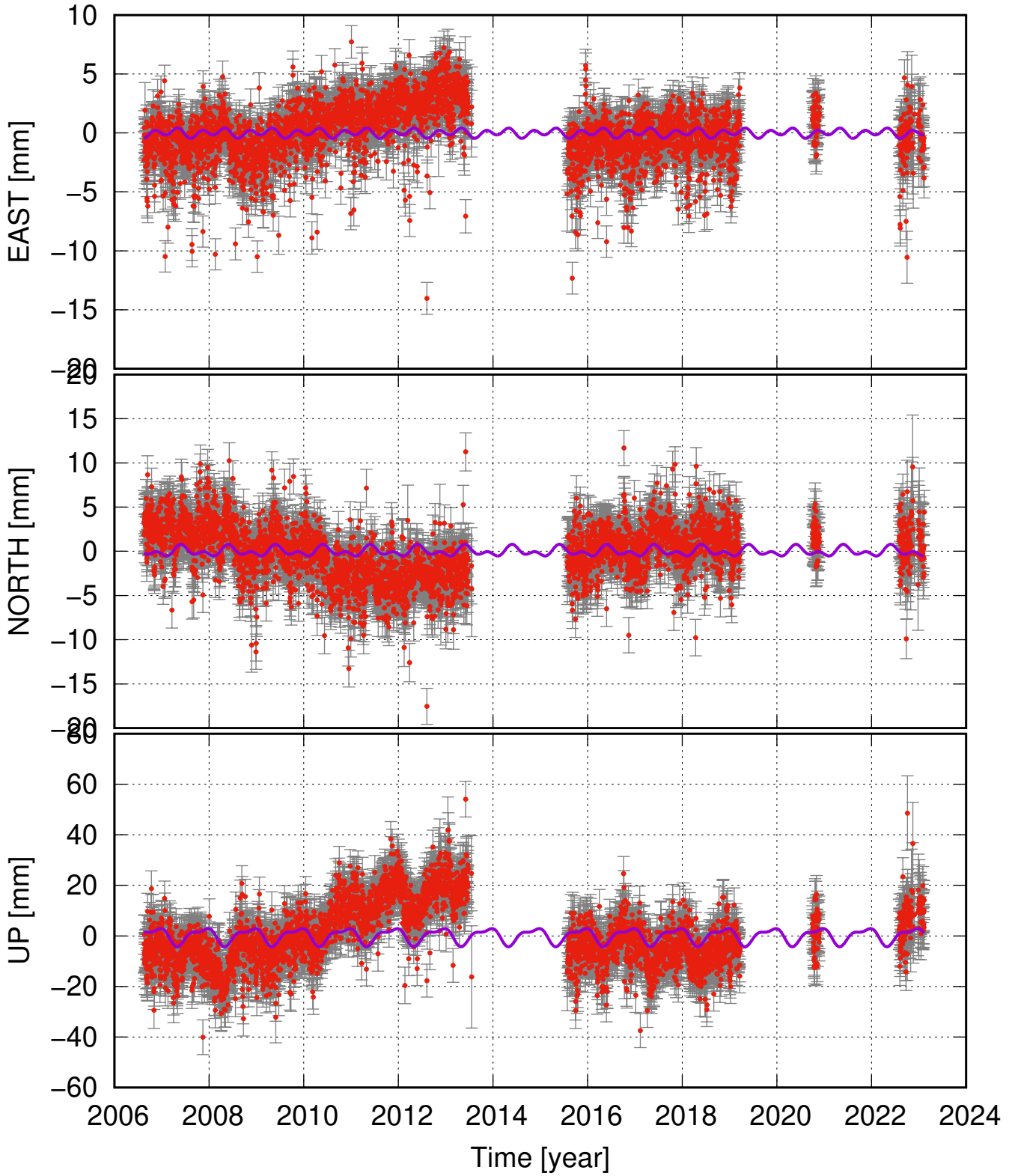
LFEL seasonal fit
