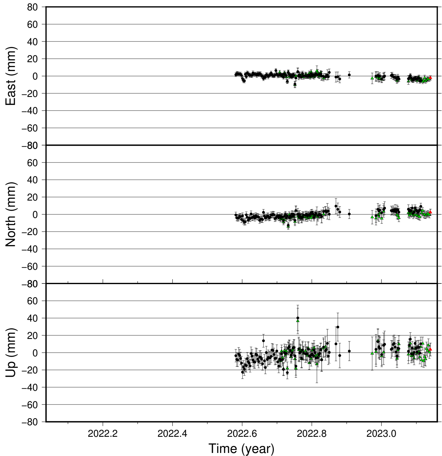
LFEL time series (IGS 2014), last 400 days
