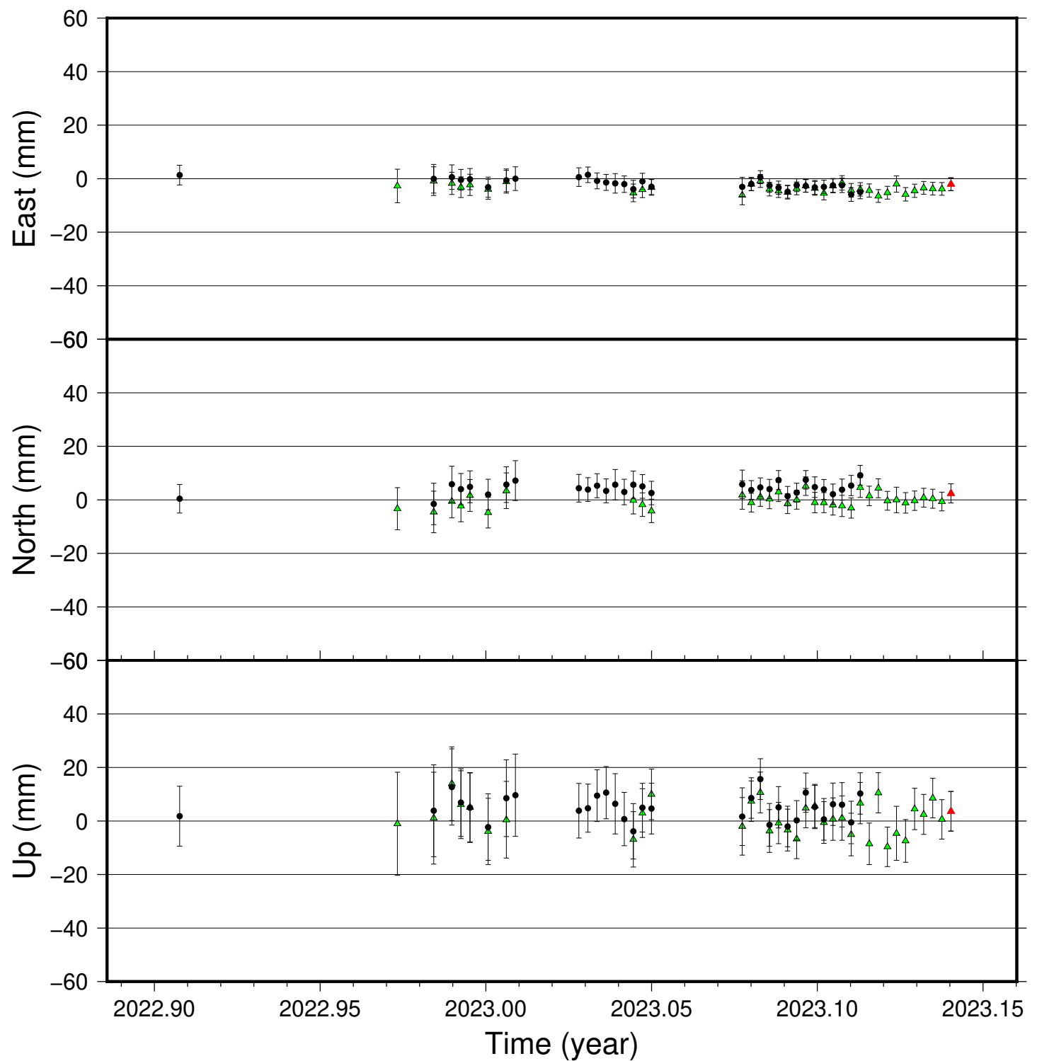
LFEL time series (IGS 2014), last 100 days
