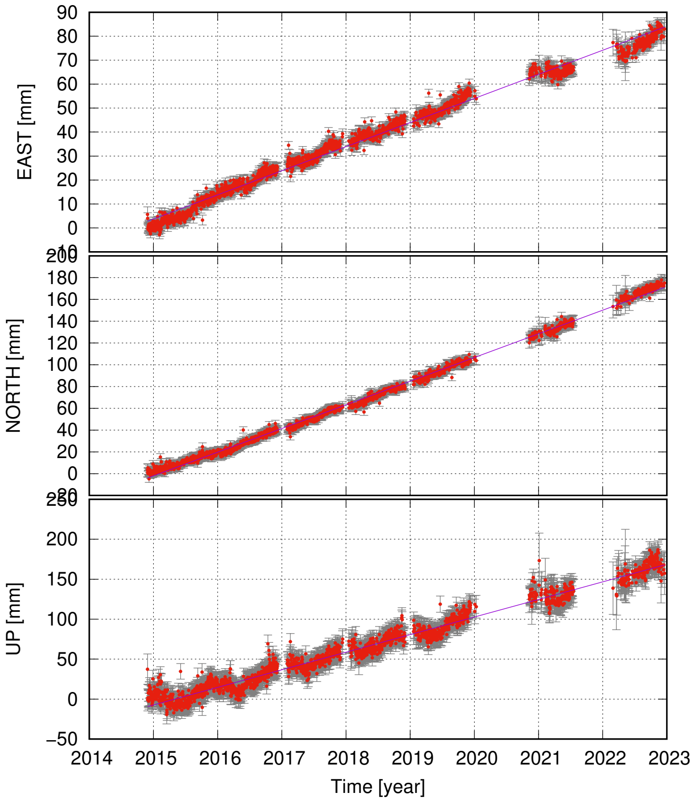
LANH (64.89, -16.56) time series (ITRF 2014) v_e = 10.06 \pm 0.31 ; v_n = 21.73 \pm 0.35 ; v_u = 21.99 \pm 1.04 mm/yr
