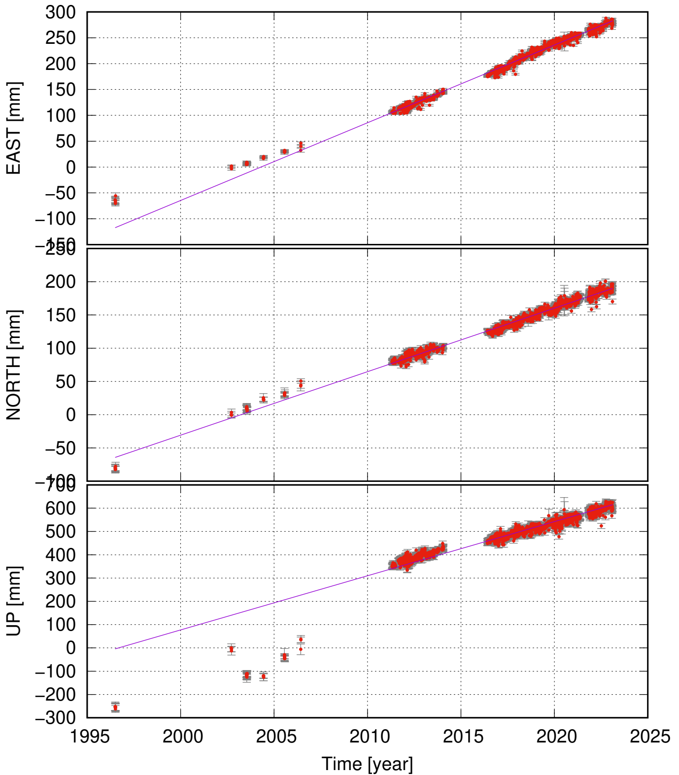
KVSK (63.98, -16.43) time series (ITRF 2014) v_e = 15.03 \pm 0.18 ; v_n = 9.55 \pm 0.14 ; v_u = 23.26 \pm 1.23 mm/yr
