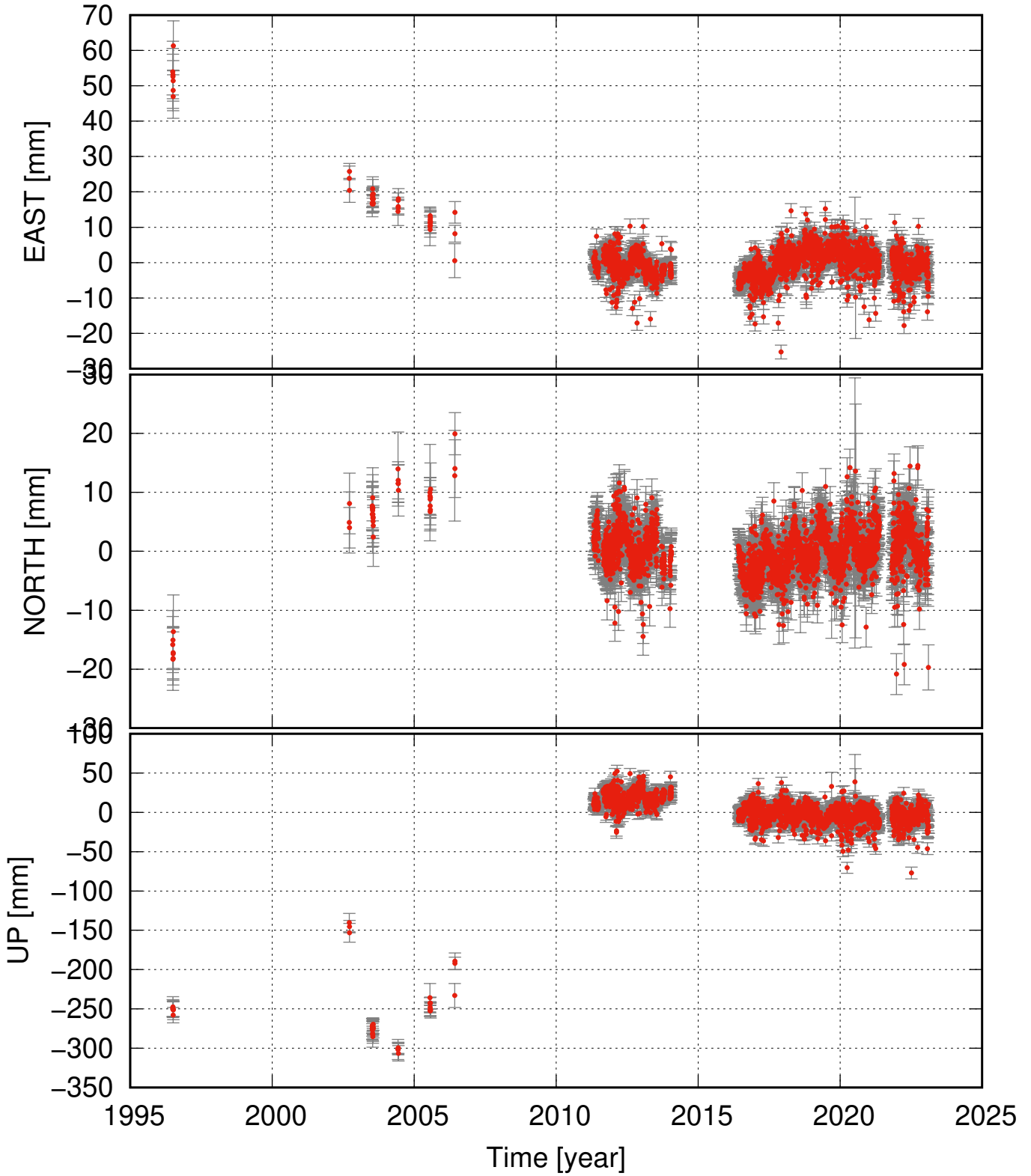
KVSK residual time series
