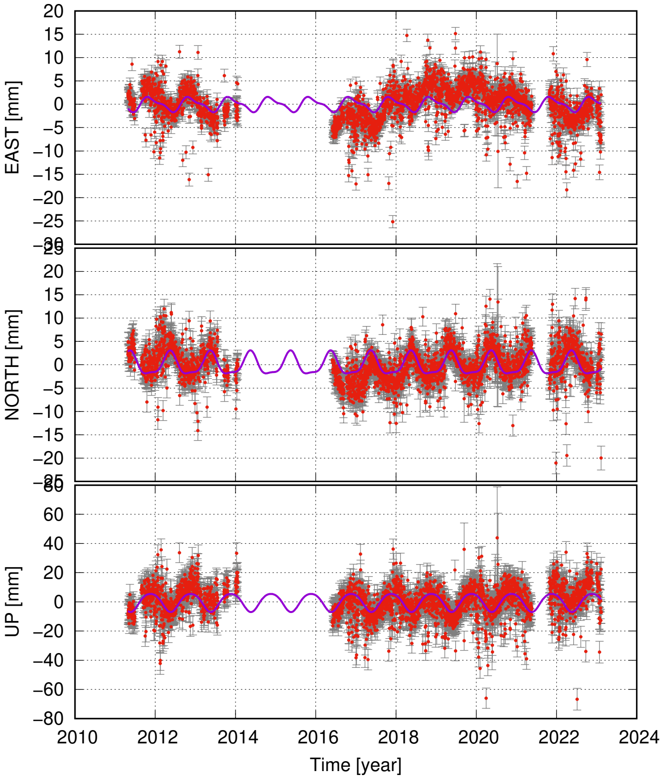
KVSK seasonal fit
