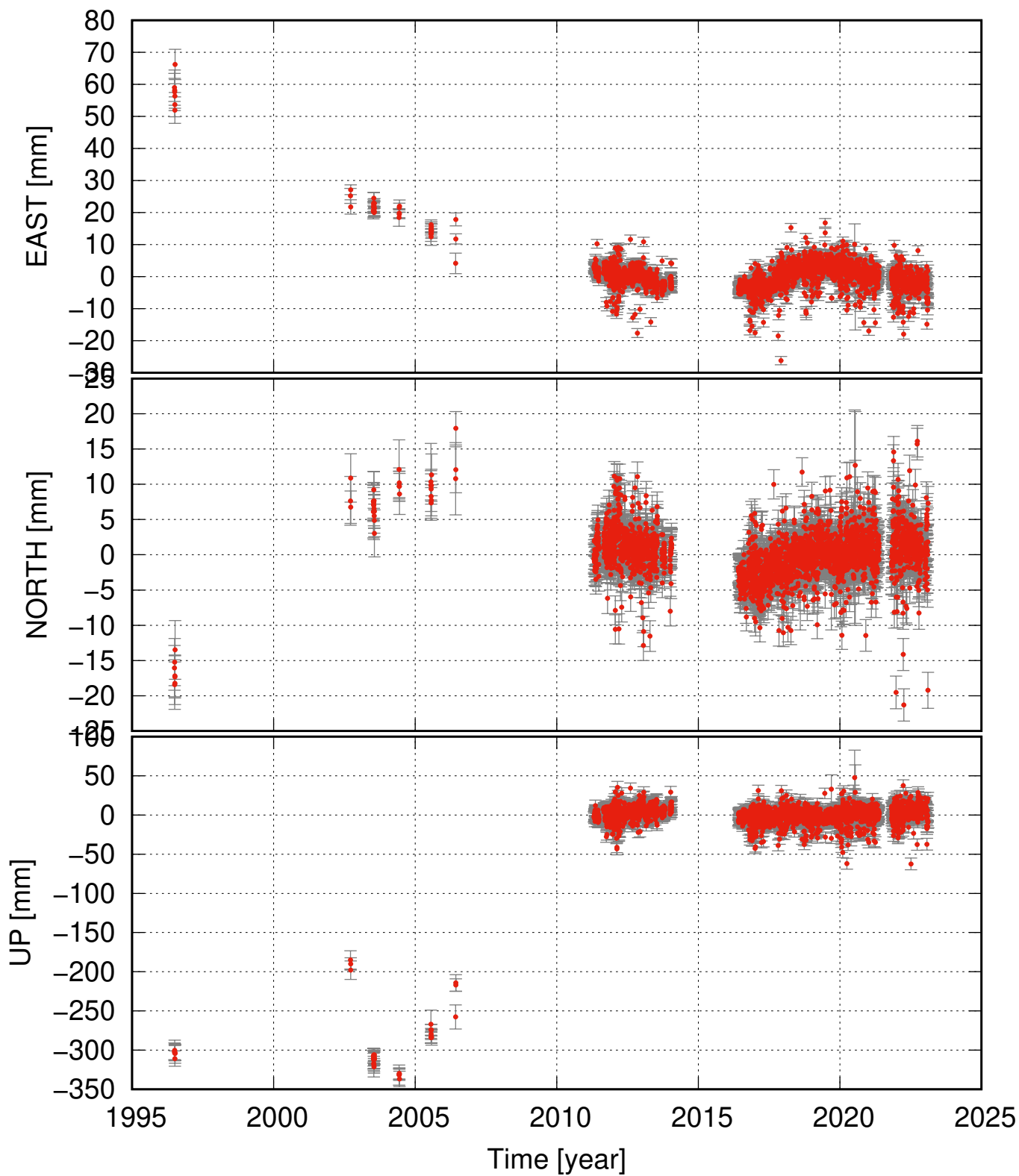
KVSK detrended and seasonal signal removed
