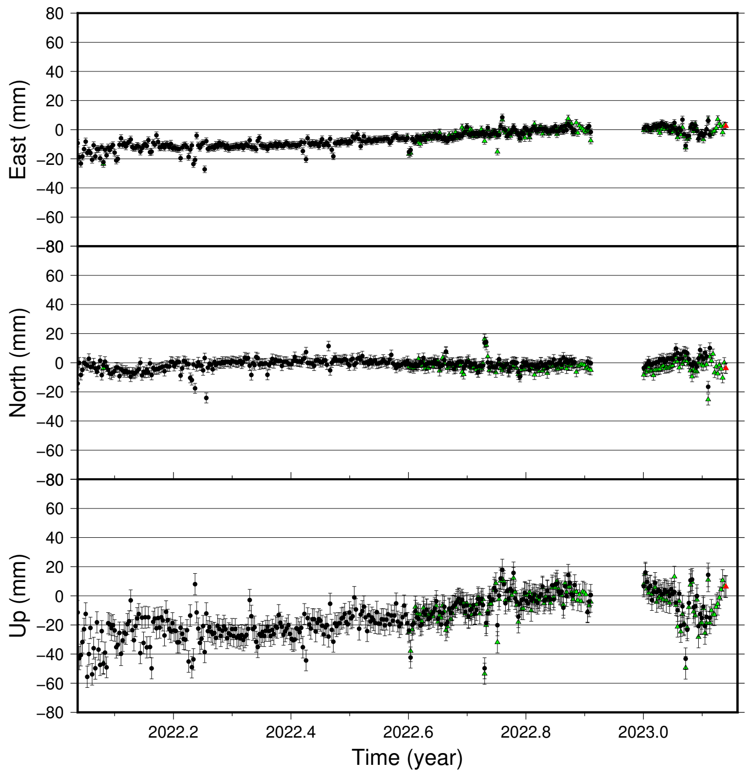
KVSK time series (IGS 2014), last 400 days
