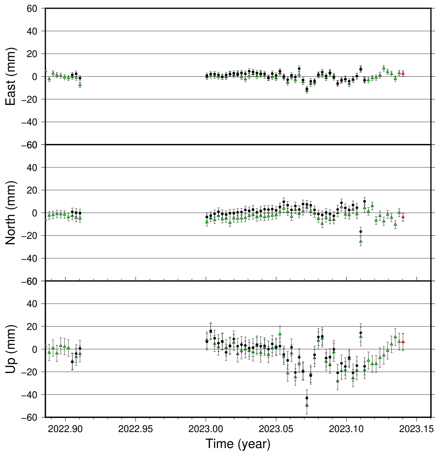
KVSK time series (IGS 2014), last 100 days
